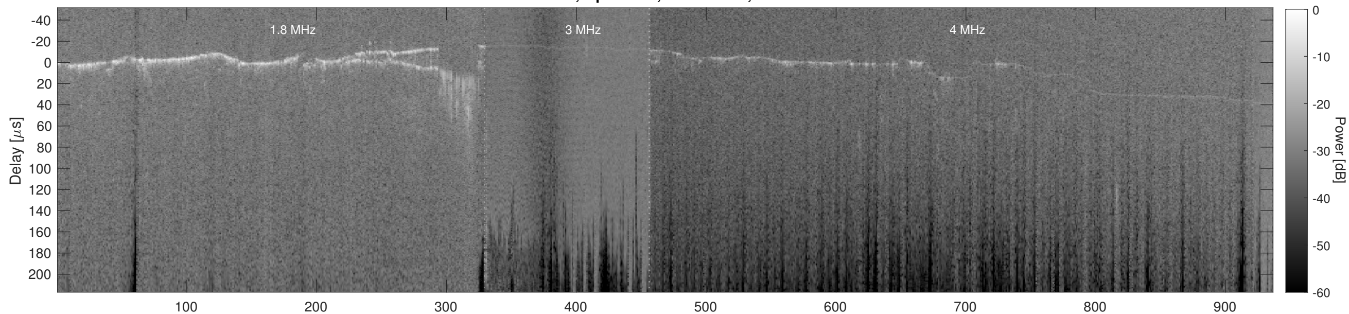
Orbit 2603, Cluttergram
