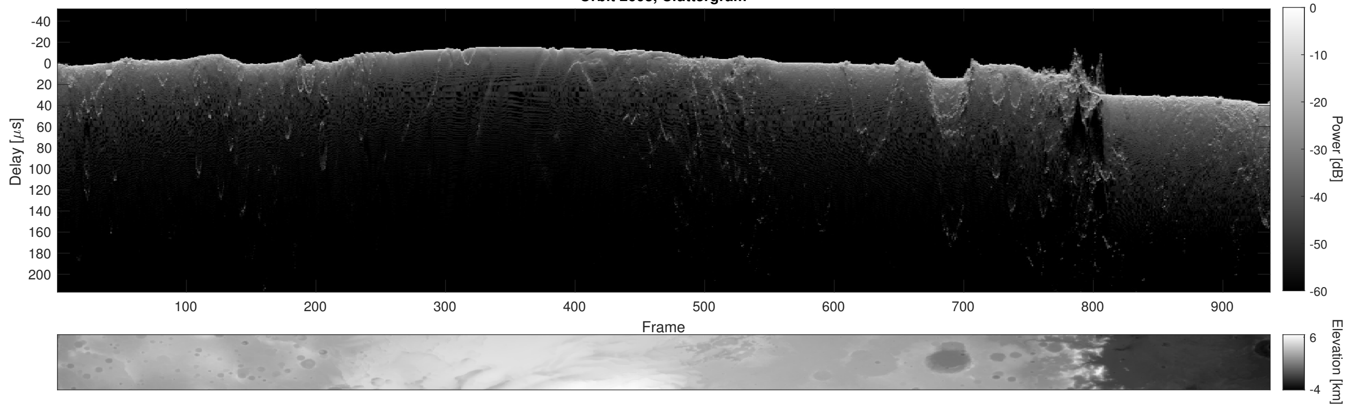
Orbit 2603, Cluttergram
