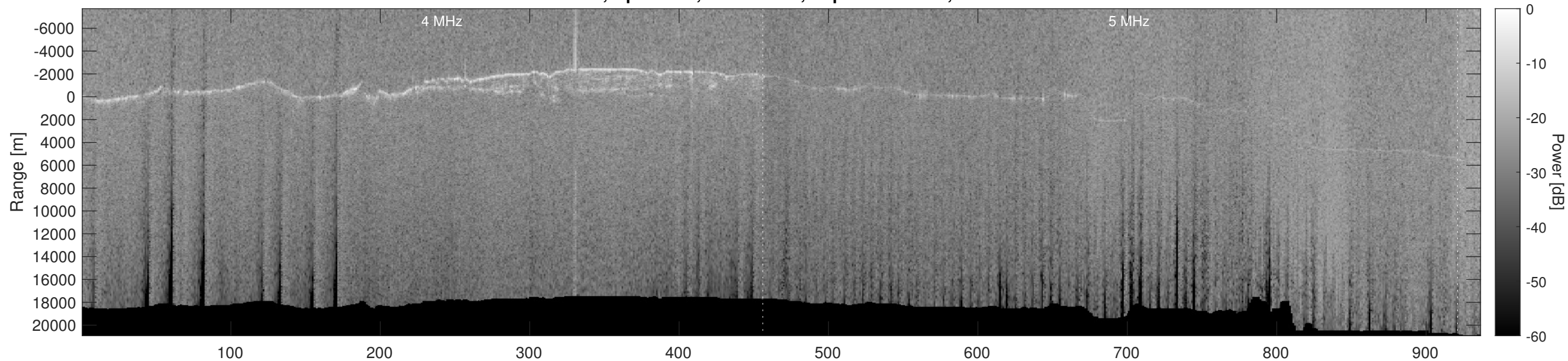
Orbit 2603, Optimized, No Window, Depth-Corrected, Channel 2
