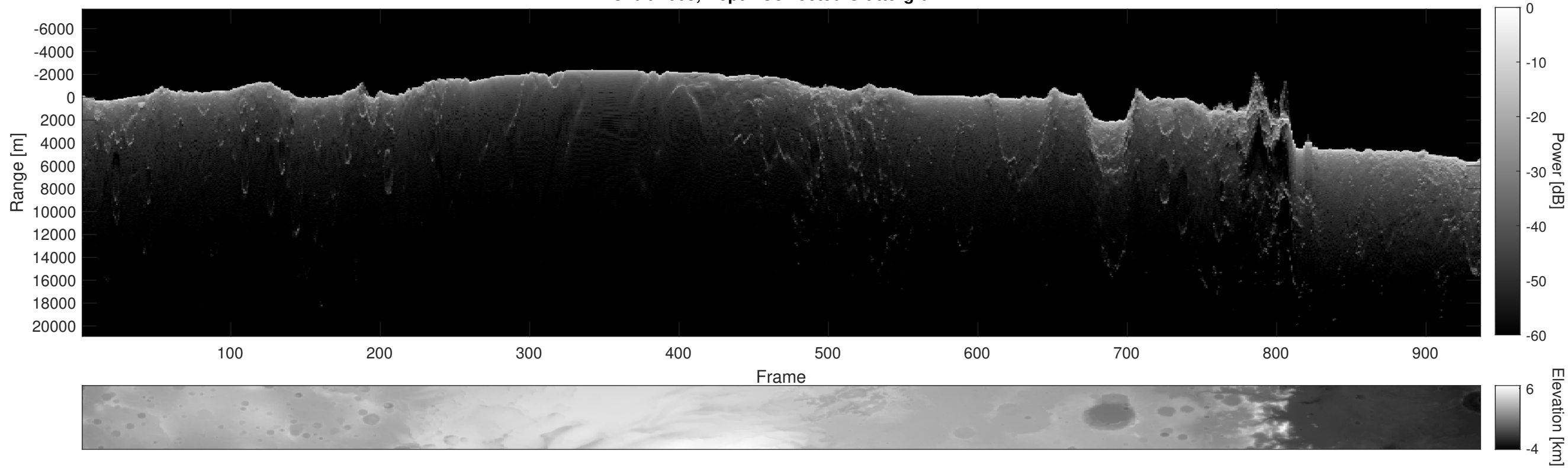
Orbit 2603, Depth-Corrected Cluttergram
