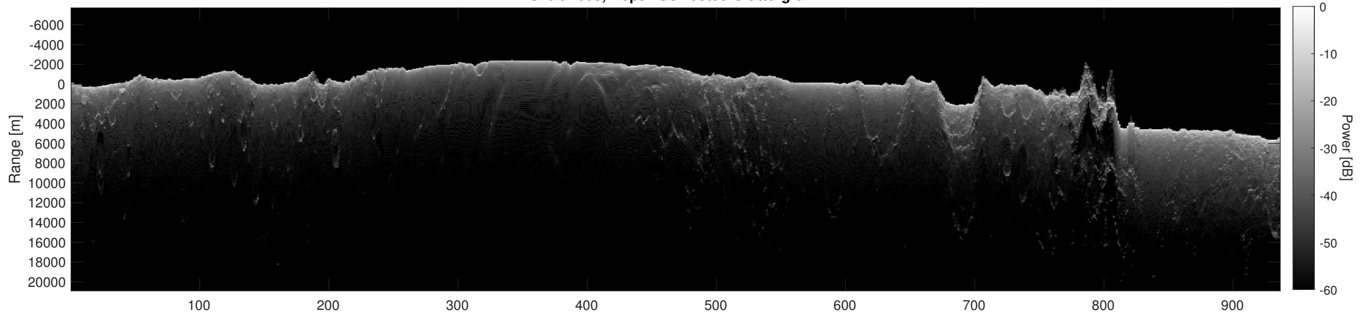
Orbit 2603, Depth-Corrected Cluttergram
