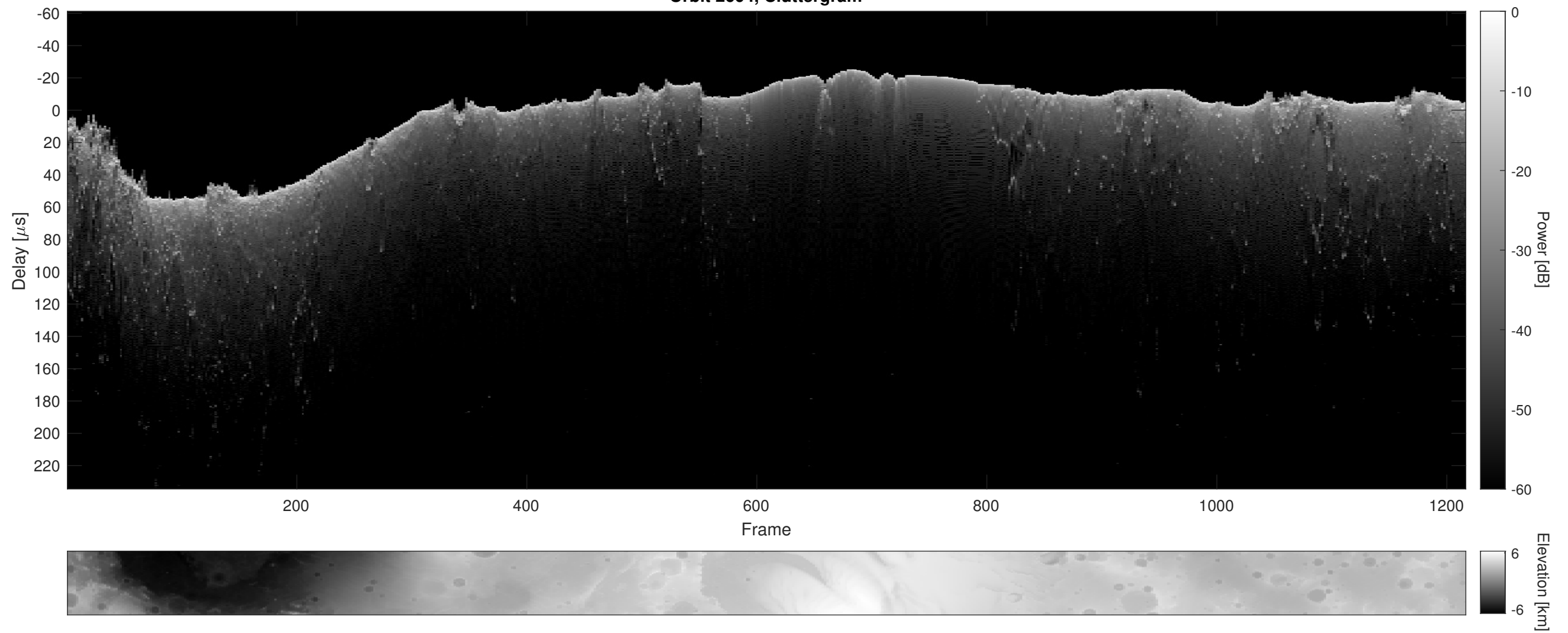
Orbit 2604, Cluttergram
