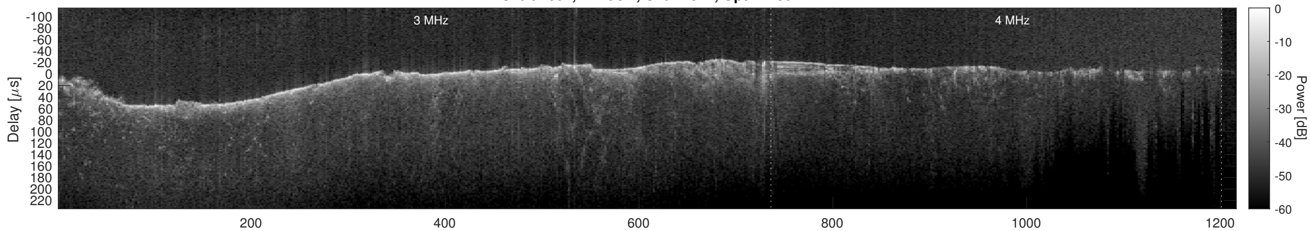
Orbit 2604, Cluttergram
