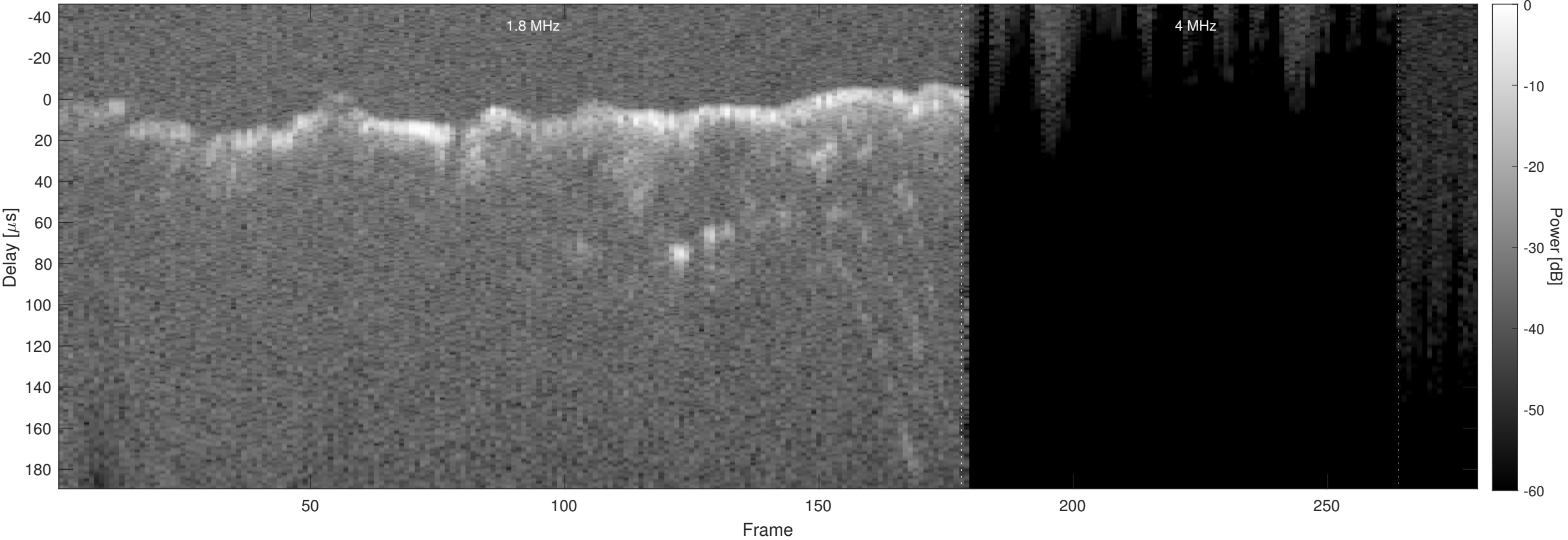
Orbit 2606, Chapman, Window, Channel 2
