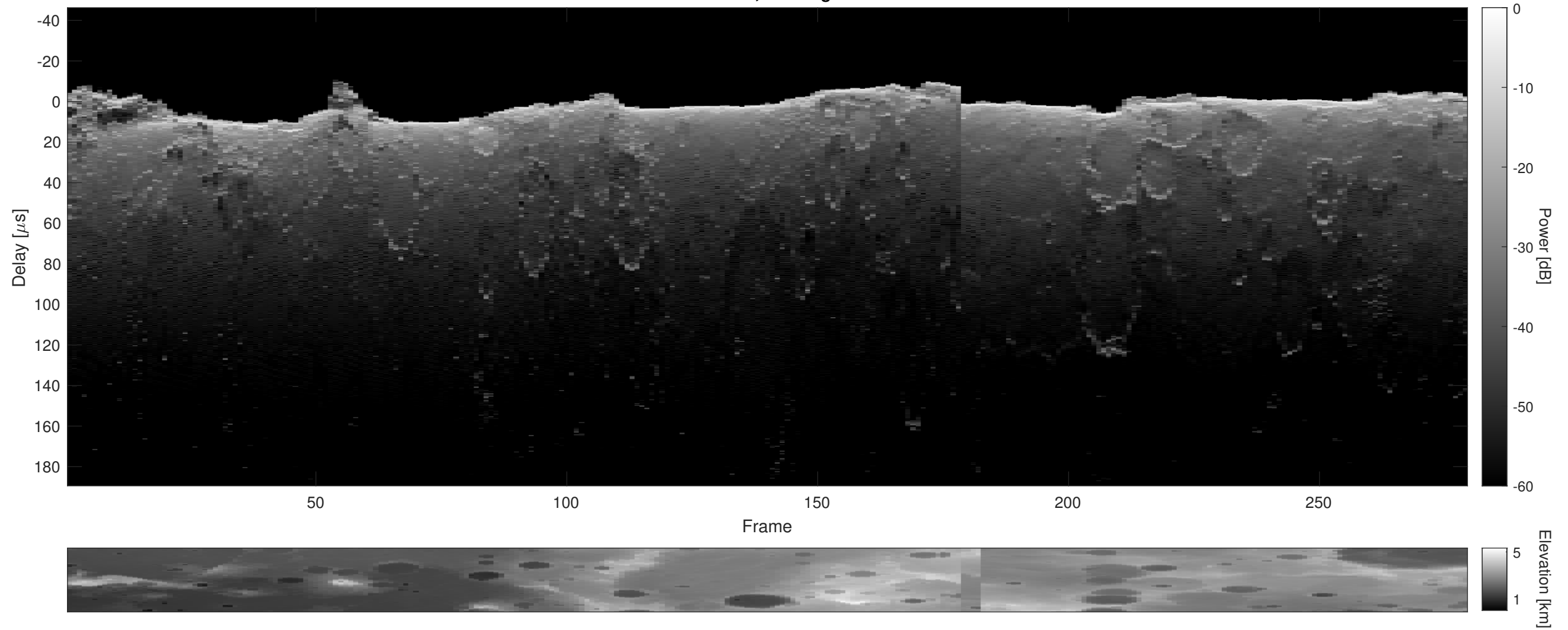
Orbit 2606, Cluttergram
