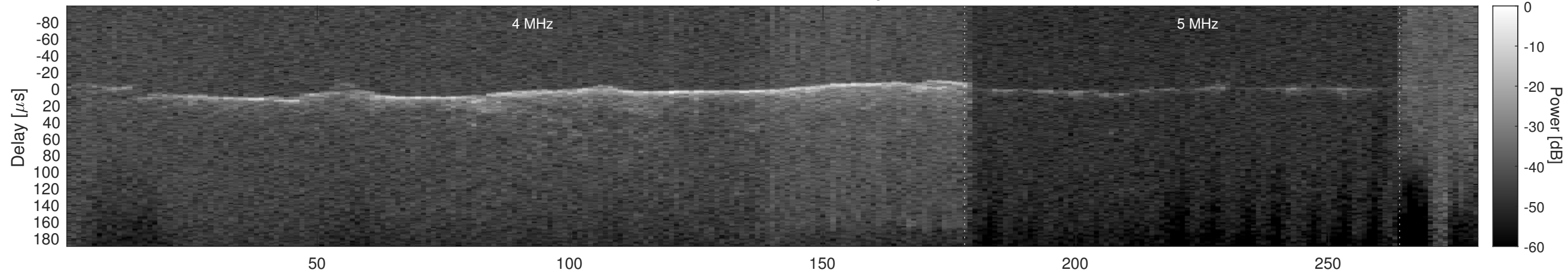
Orbit 2606, Cluttergram
