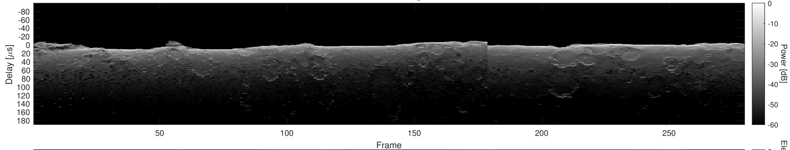
Orbit 2606, Cluttergram
