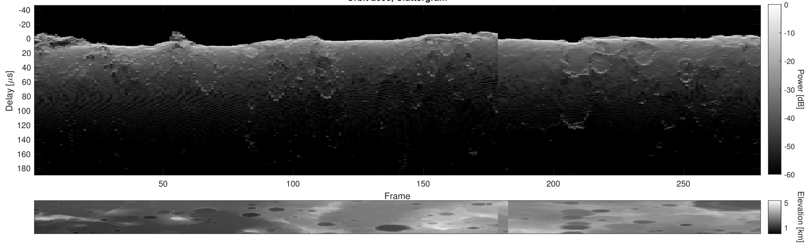
Orbit 2606, Cluttergram
