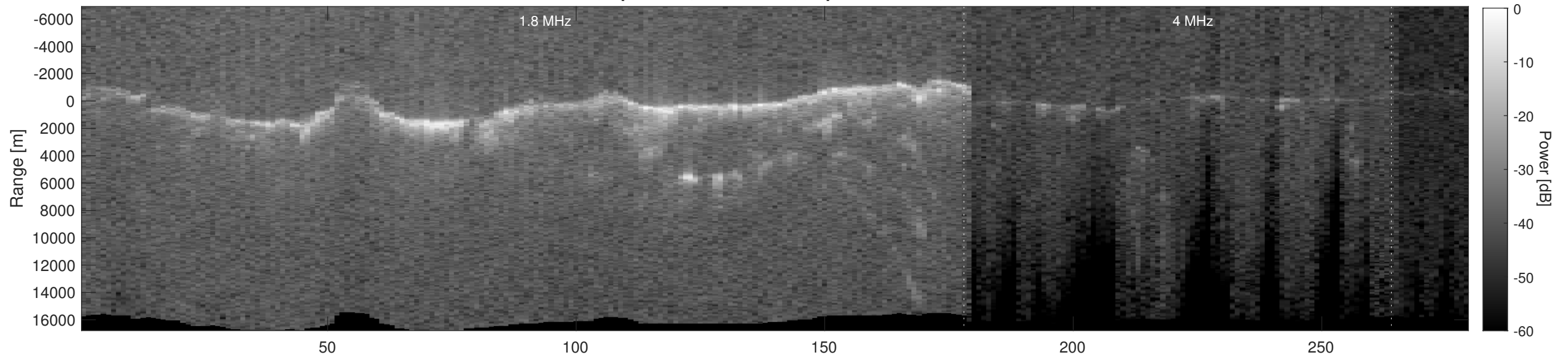
Orbit 2606, Depth-Corrected Cluttergram
