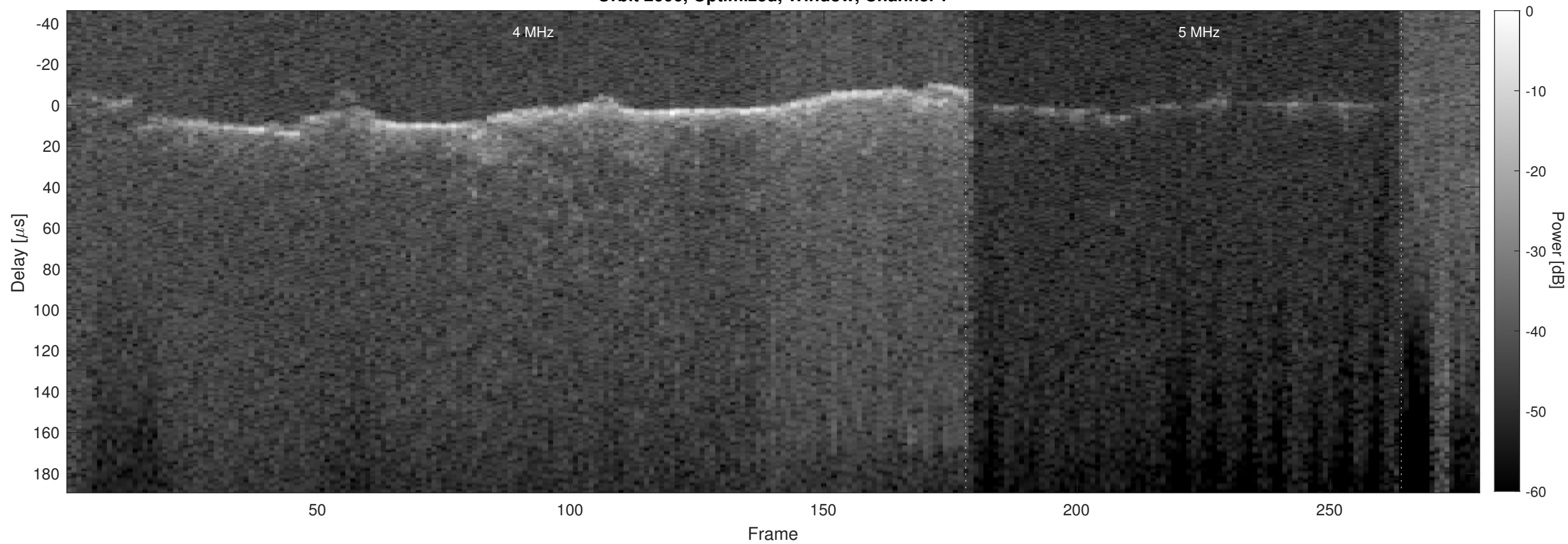
Orbit 2606, Optimized, Window, Channel 2
