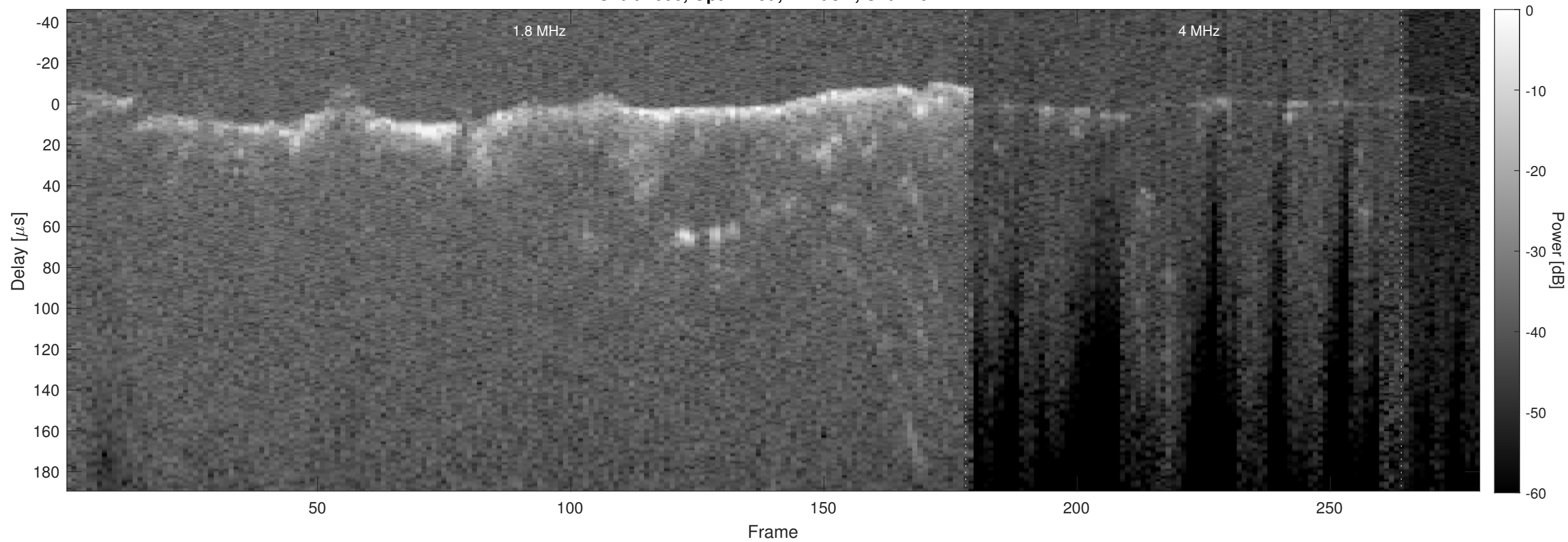
Orbit 2606, Optimized, Window, Channel 2
