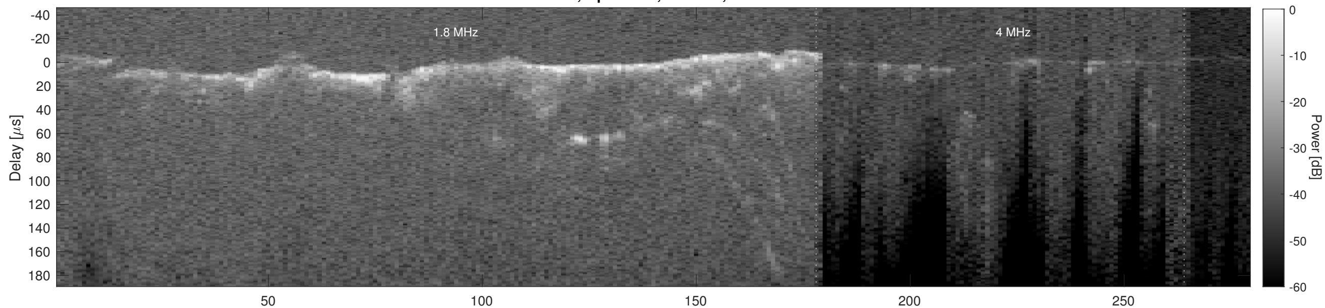
Orbit 2606, Cluttergram
