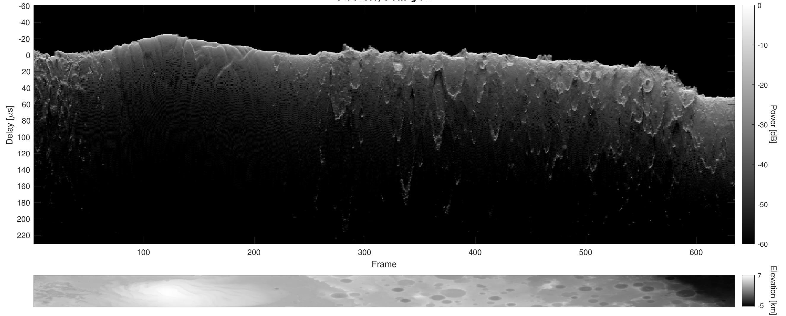
Orbit 2609, Cluttergram
