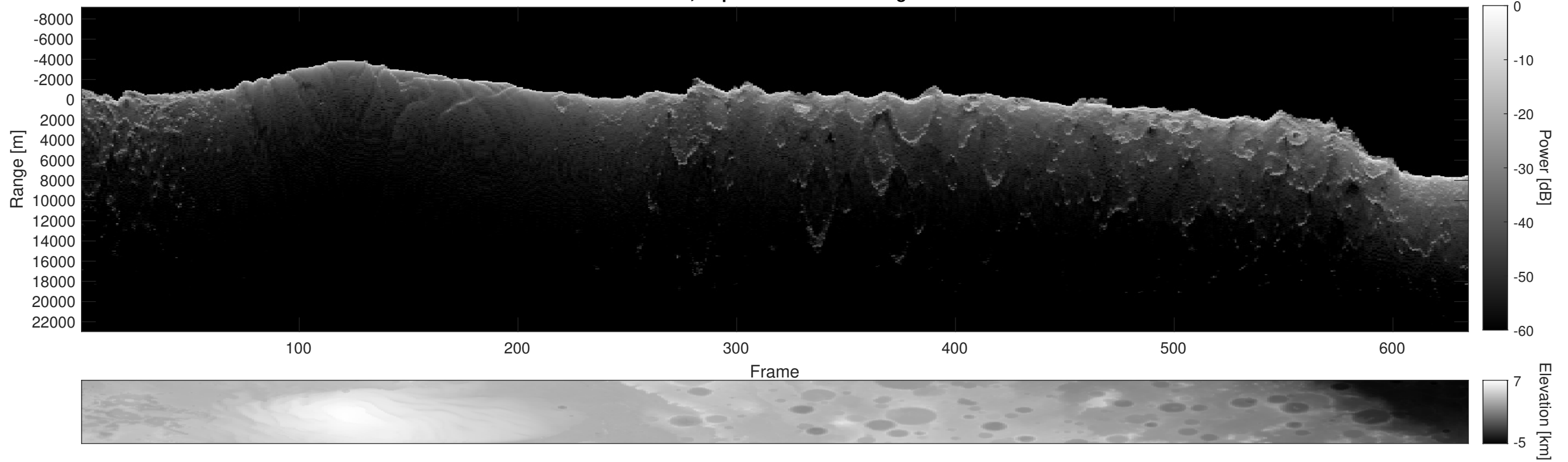
Orbit 2609, Depth-Corrected Cluttergram
