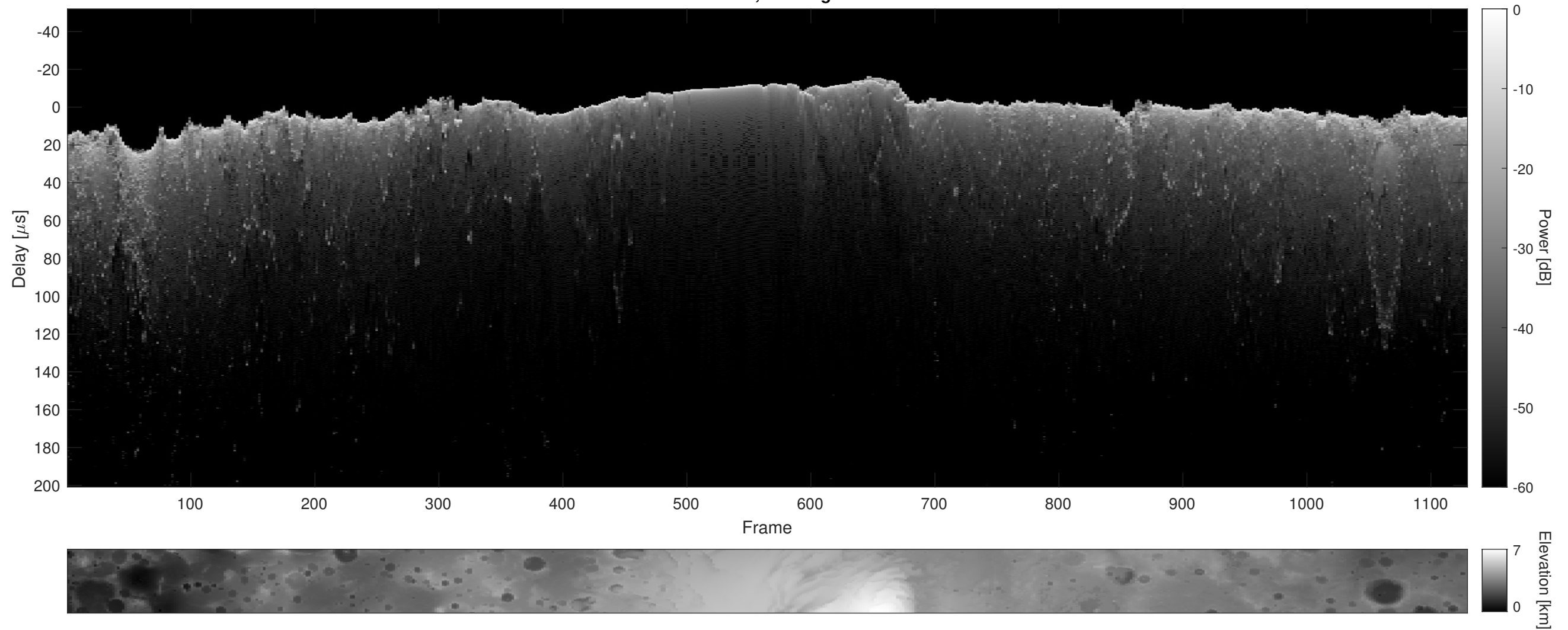
Orbit 2610, Cluttergram
