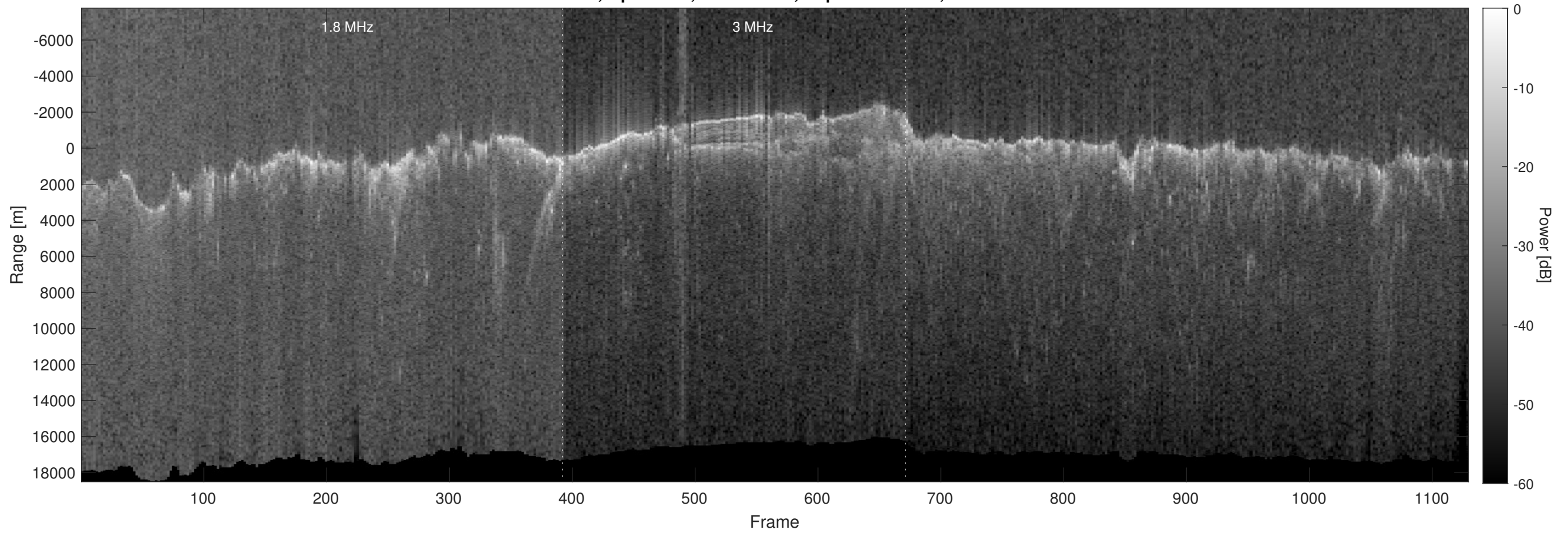
Orbit 2610, Optimized, No Window, Depth-Corrected, Channel 2
