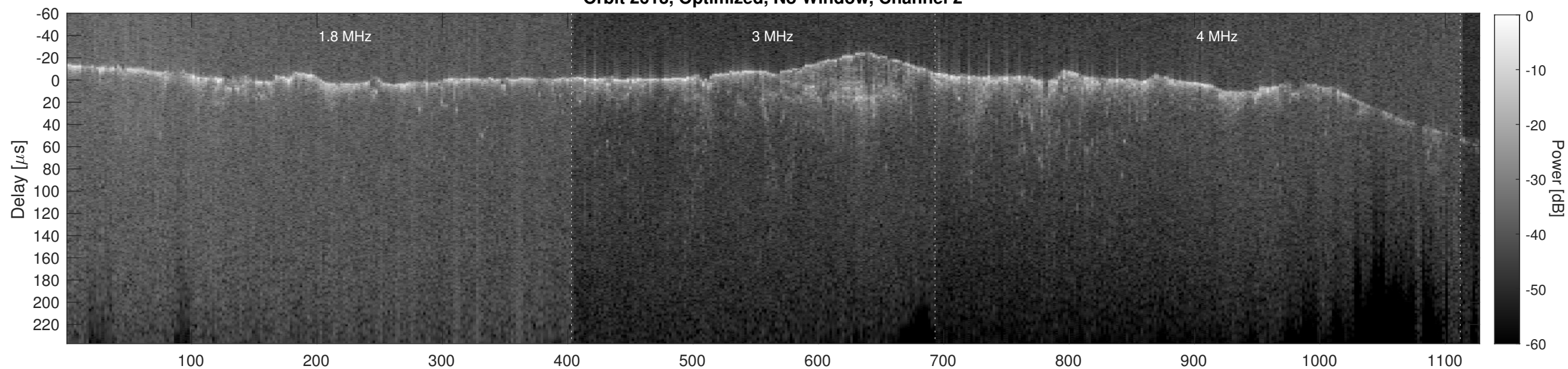
Orbit 2613, Cluttergram
