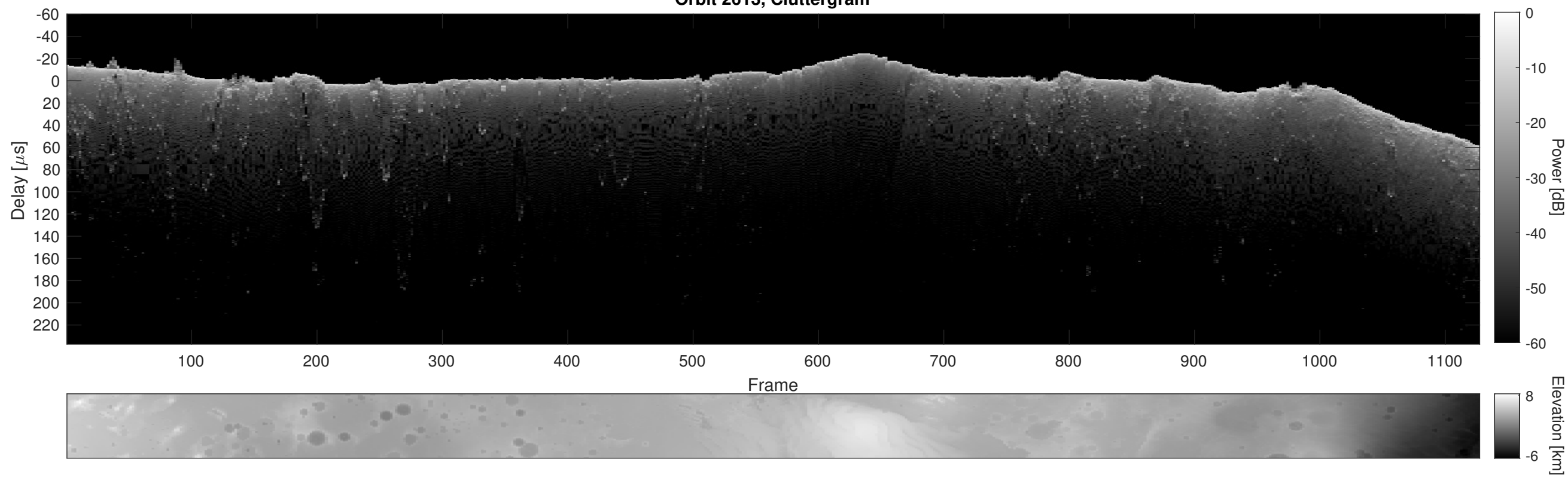
Orbit 2613, Cluttergram
