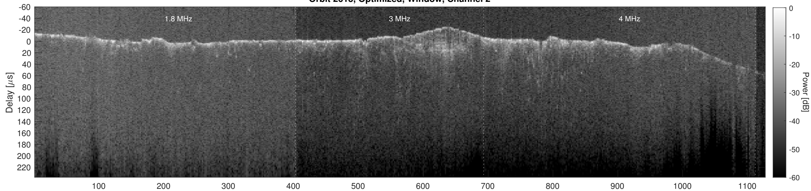
Orbit 2613, Cluttergram
