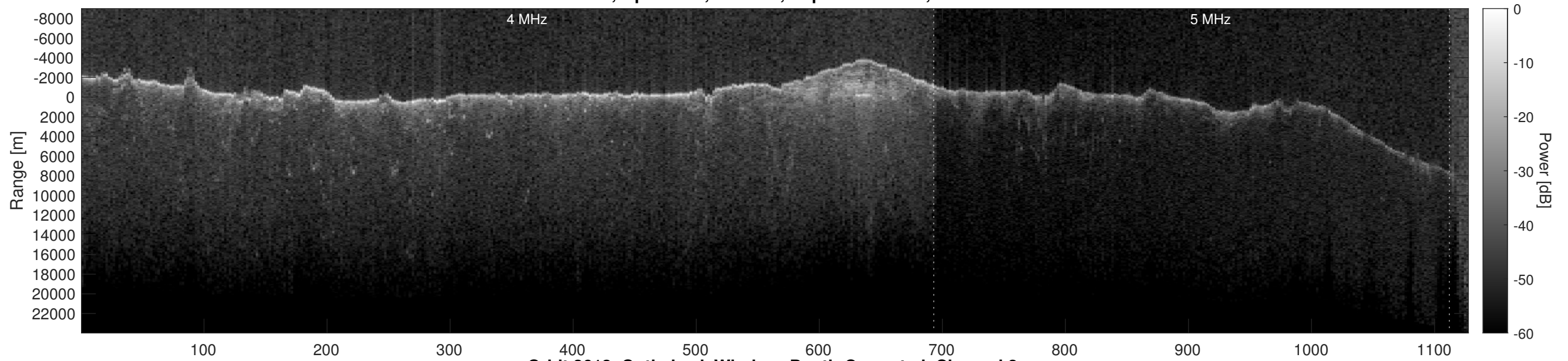
Orbit 2613, Optimized, Window, Depth-Corrected, Channel 2
