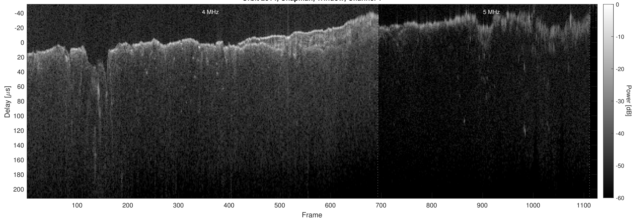
Orbit 2614, Chapman, Window, Channel 2
