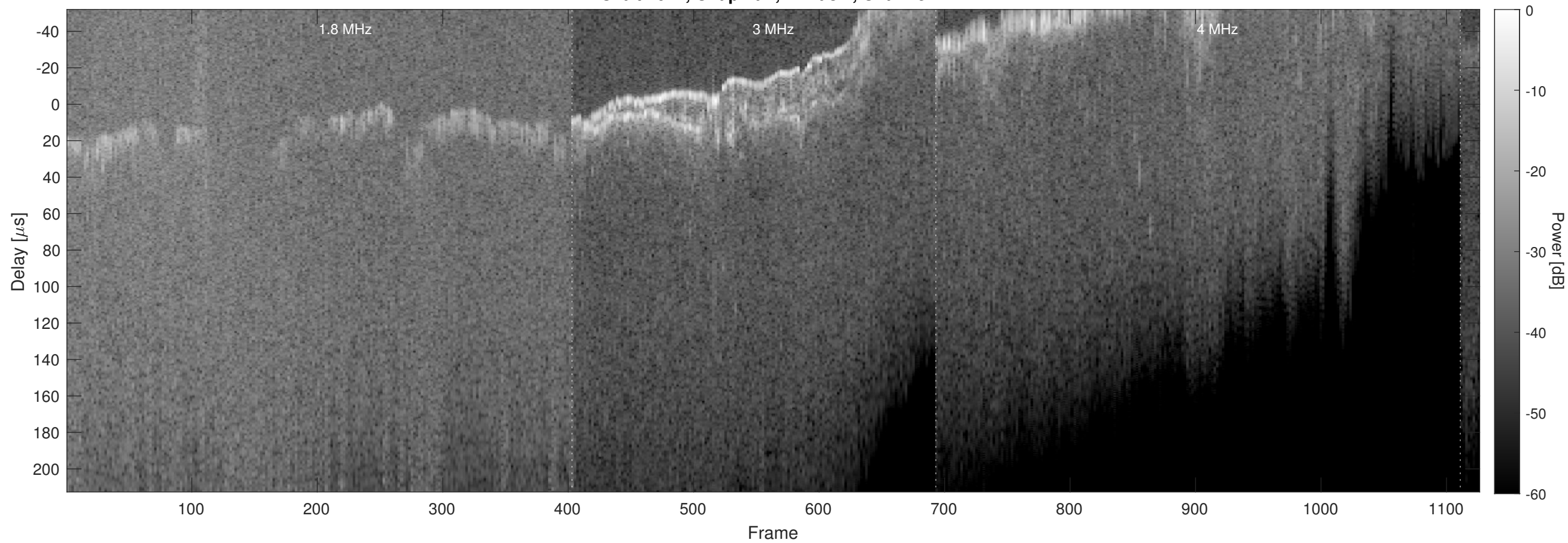
Orbit 2614, Chapman, Window, Channel 2
