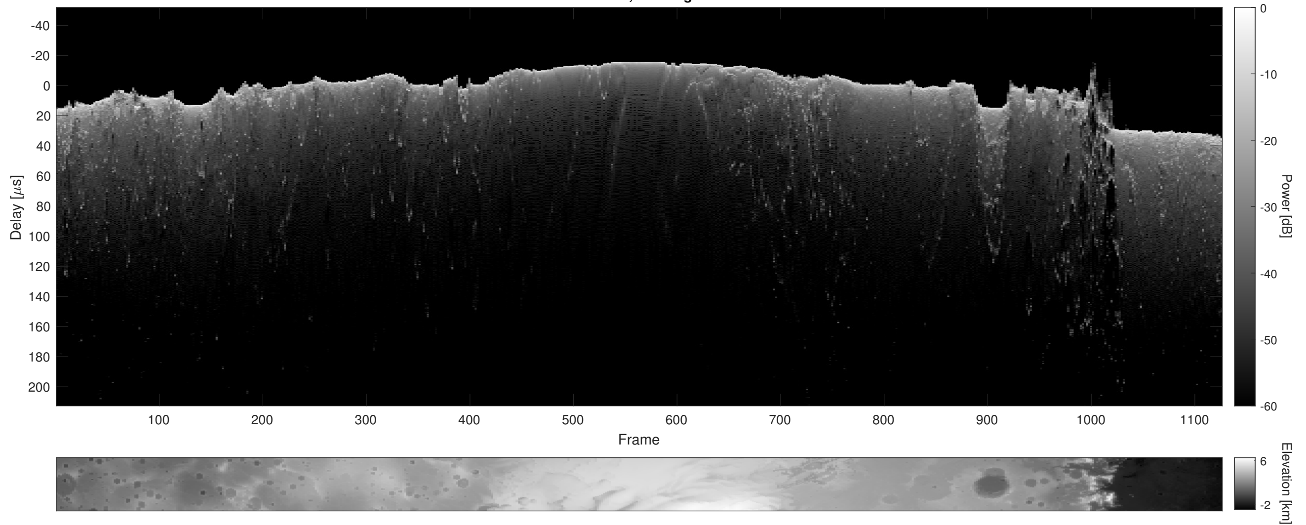
Orbit 2614, Cluttergram
