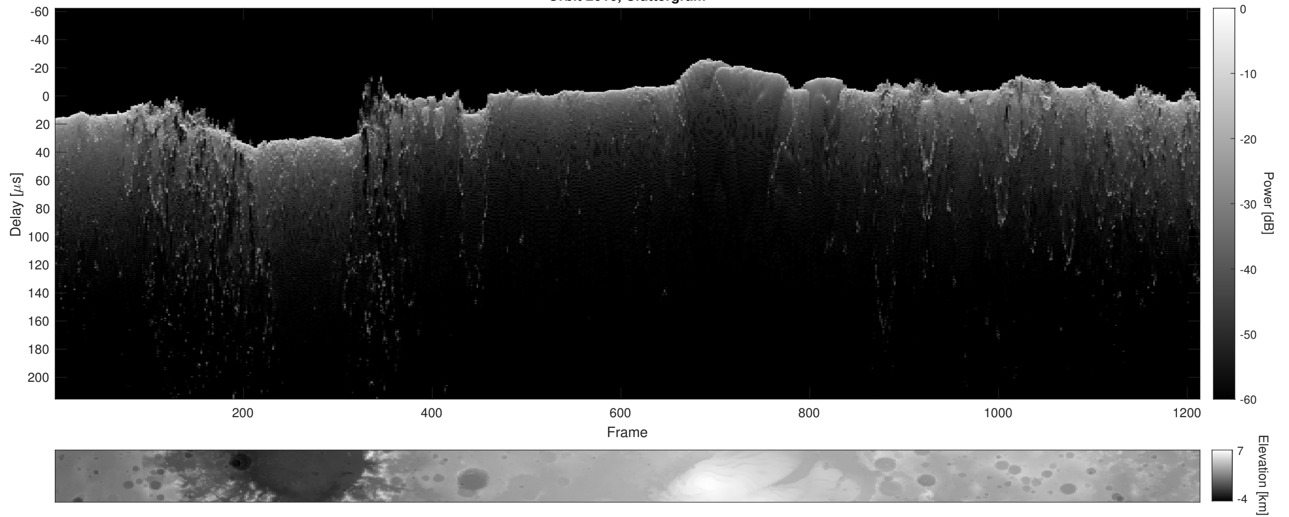
Orbit 2616, Cluttergram
