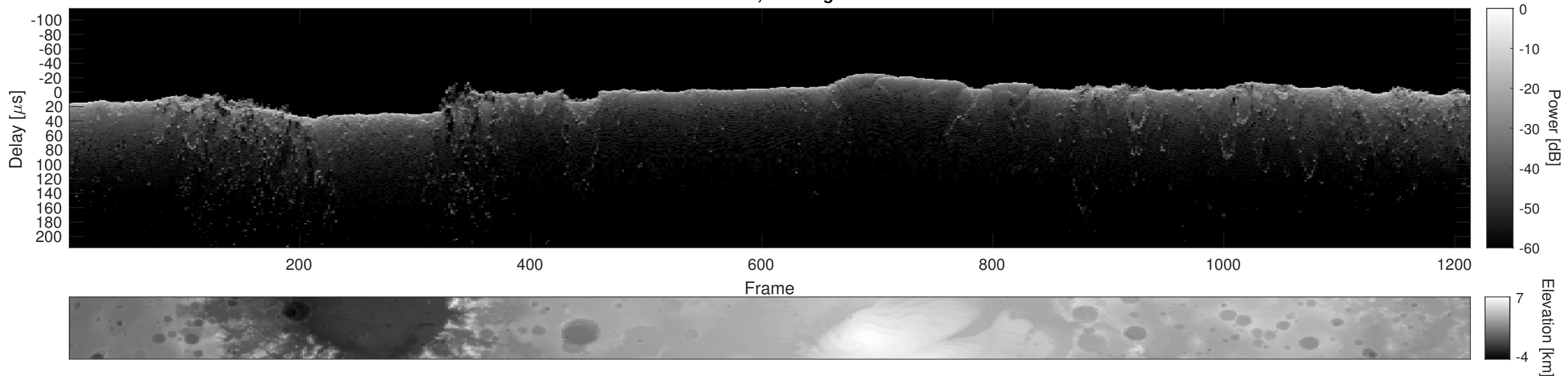
Orbit 2616, Cluttergram
