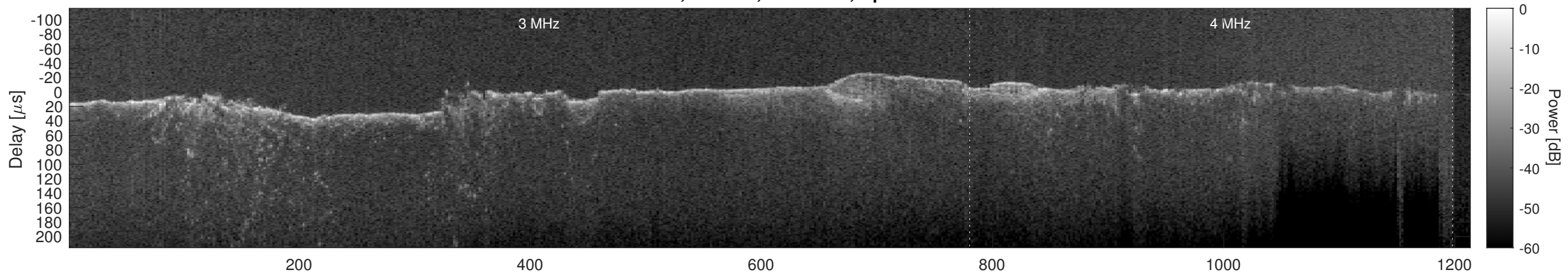
Orbit 2616, Cluttergram
