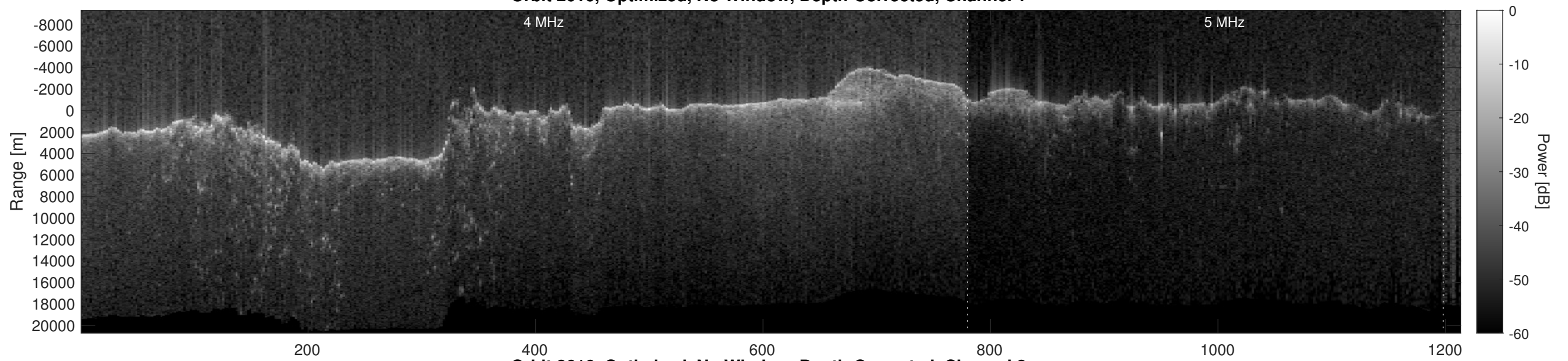
Orbit 2616, Optimized, No Window, Depth-Corrected, Channel 2
