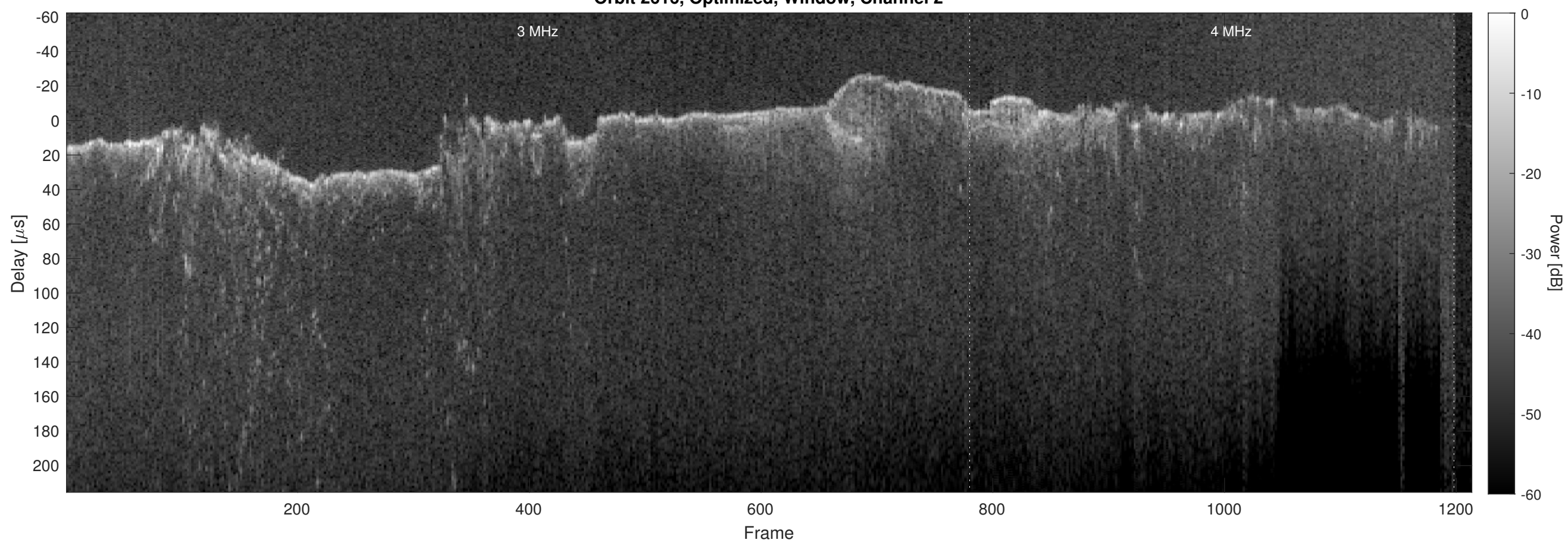
Orbit 2616, Optimized, Window, Channel 2
