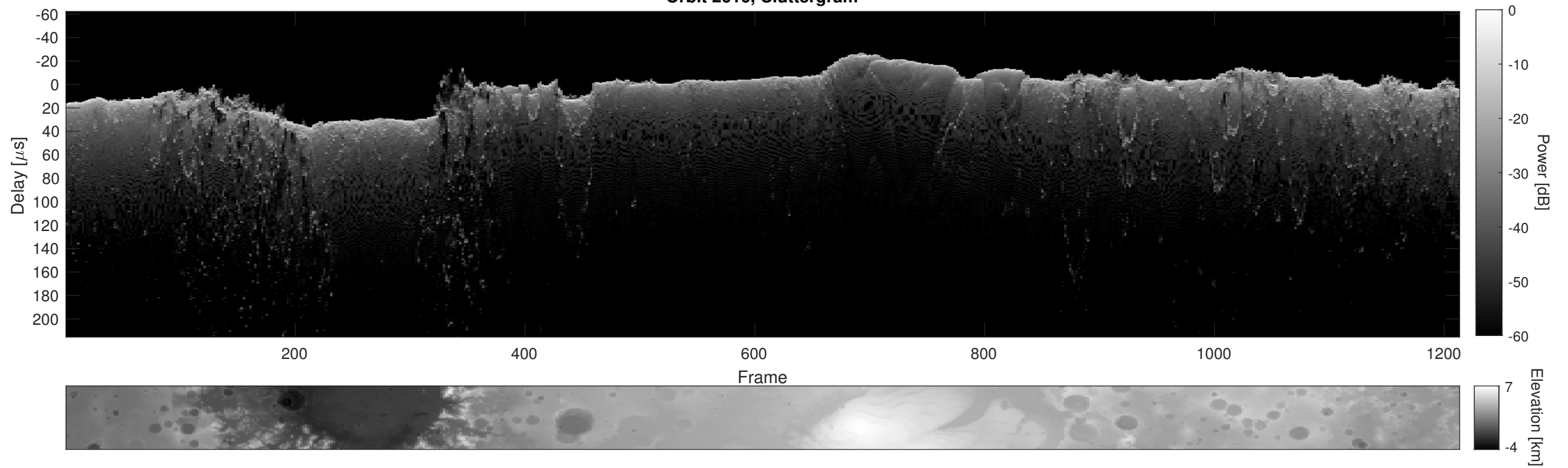
Orbit 2616, Cluttergram
