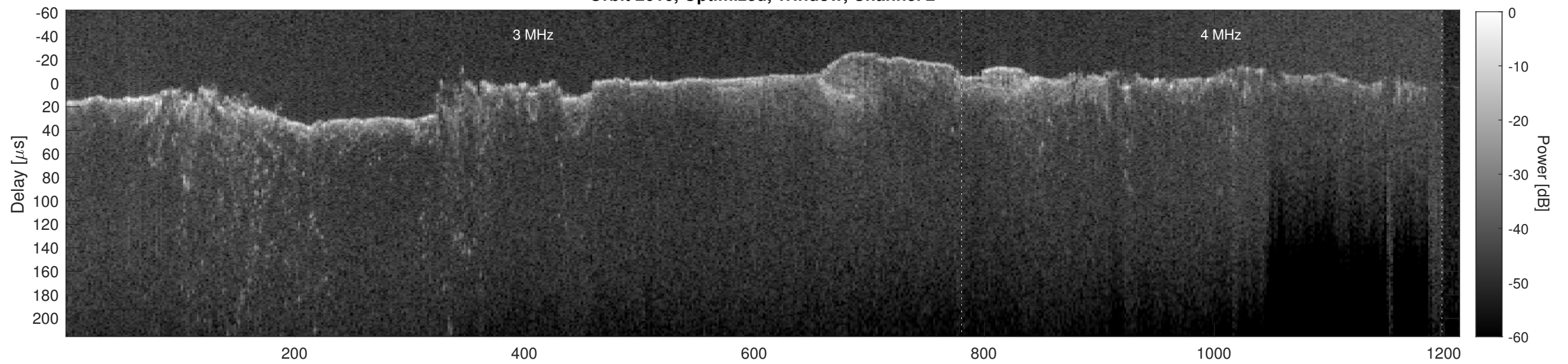
Orbit 2616, Cluttergram
