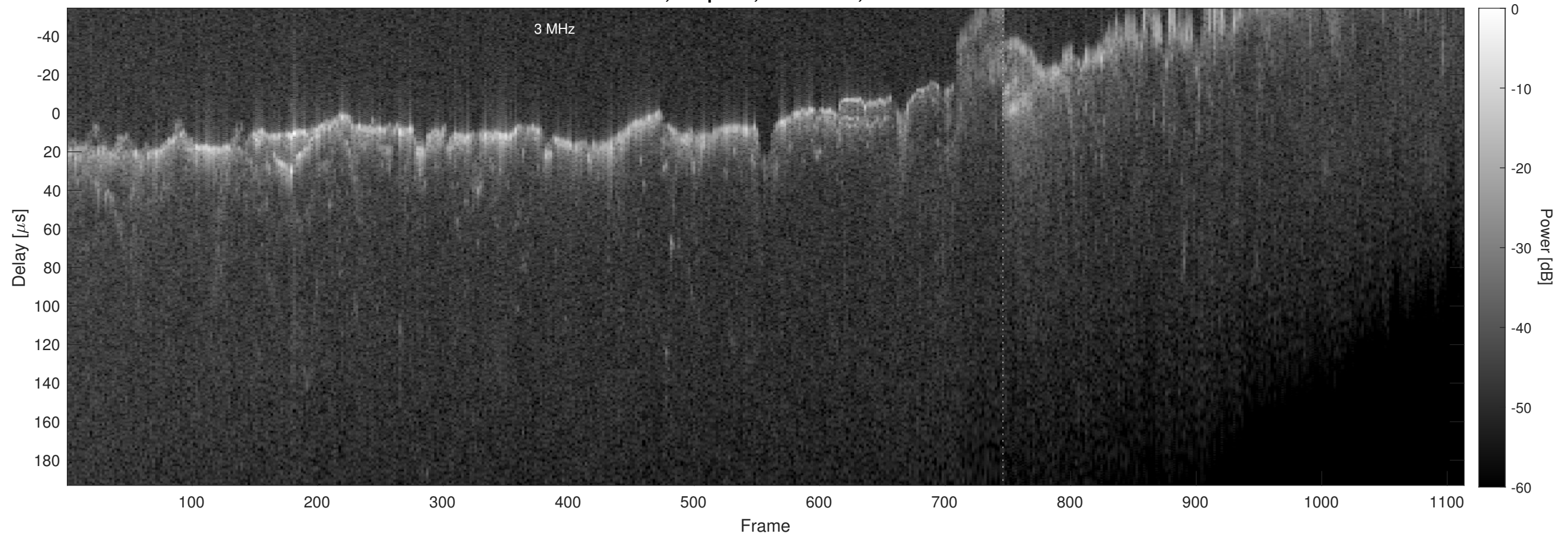
Orbit 2617, Chapman, No Window, Channel 2
