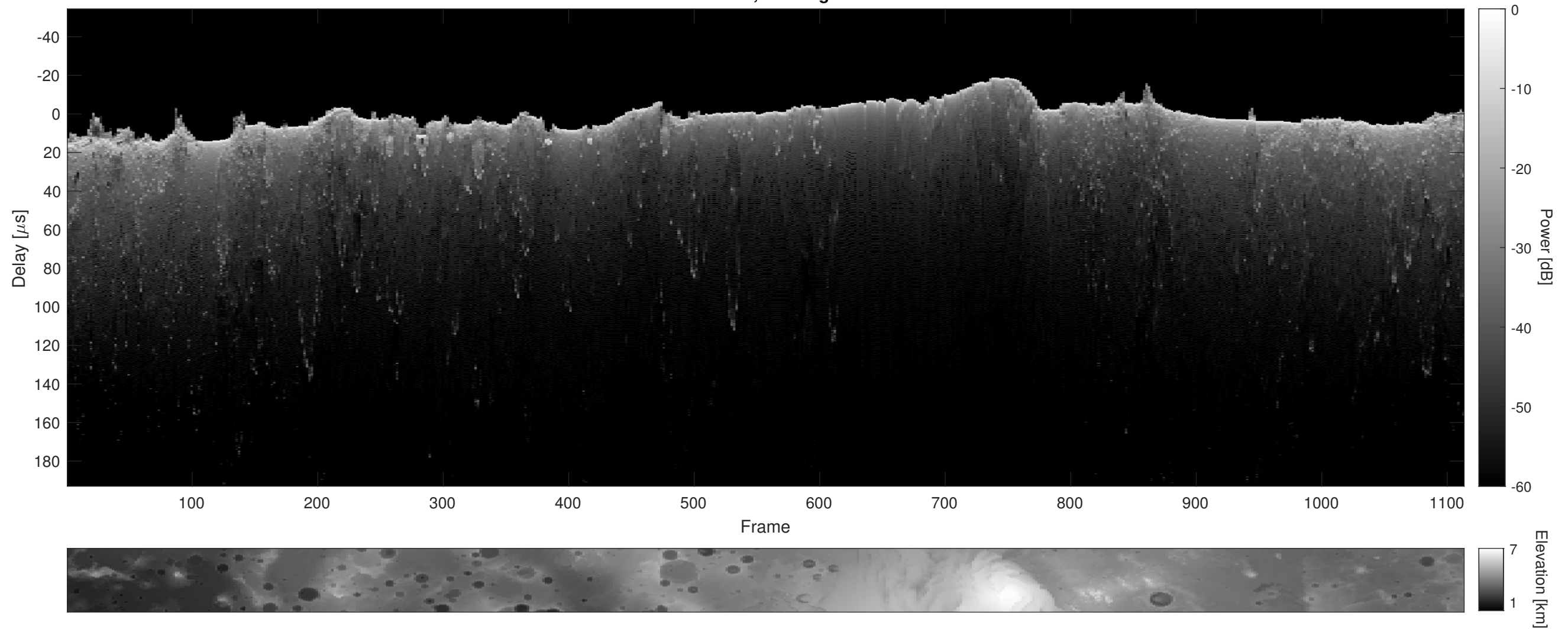
Orbit 2617, Cluttergram
