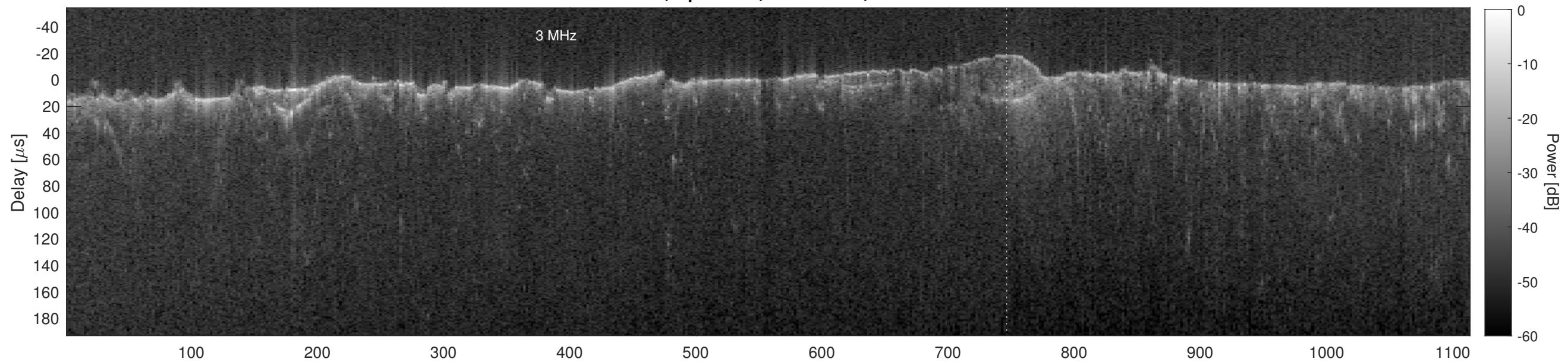
Orbit 2617, Cluttergram
