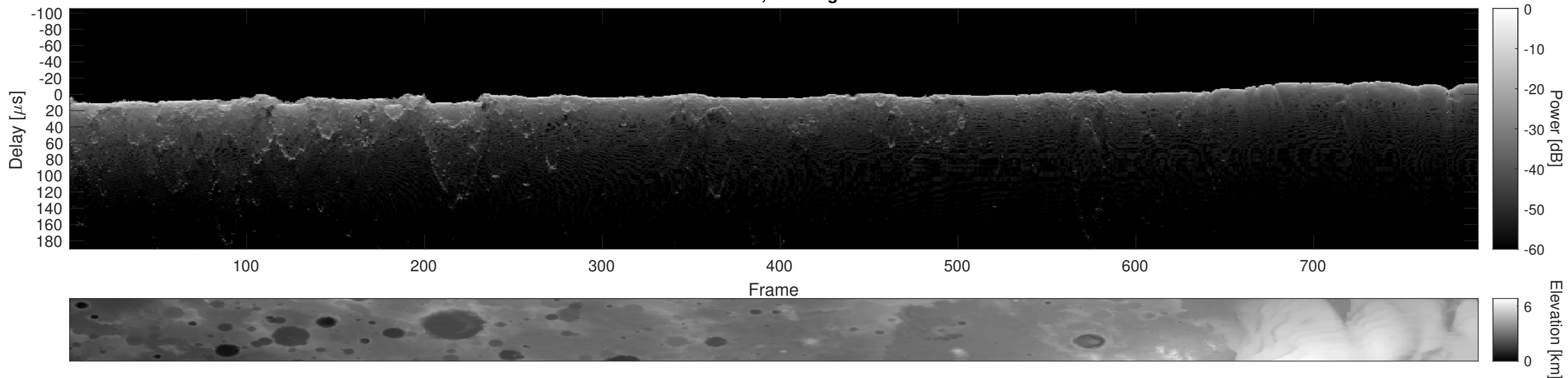
Orbit 2619, Cluttergram
