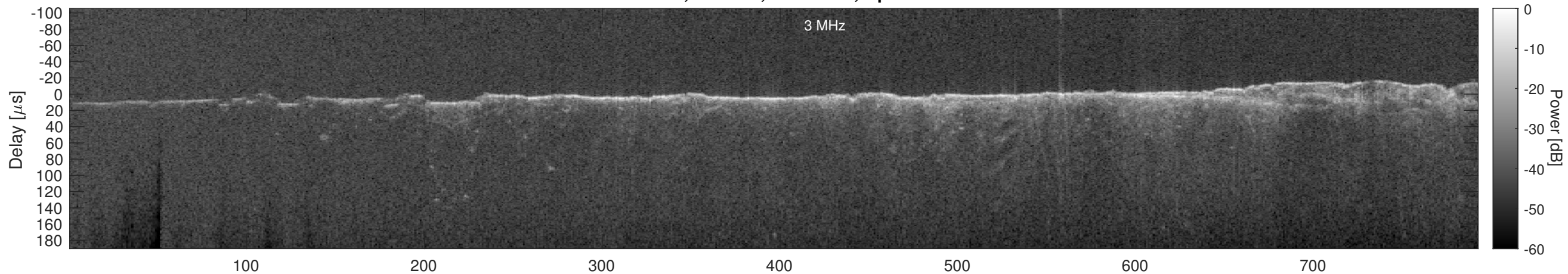
Orbit 2619, Cluttergram
