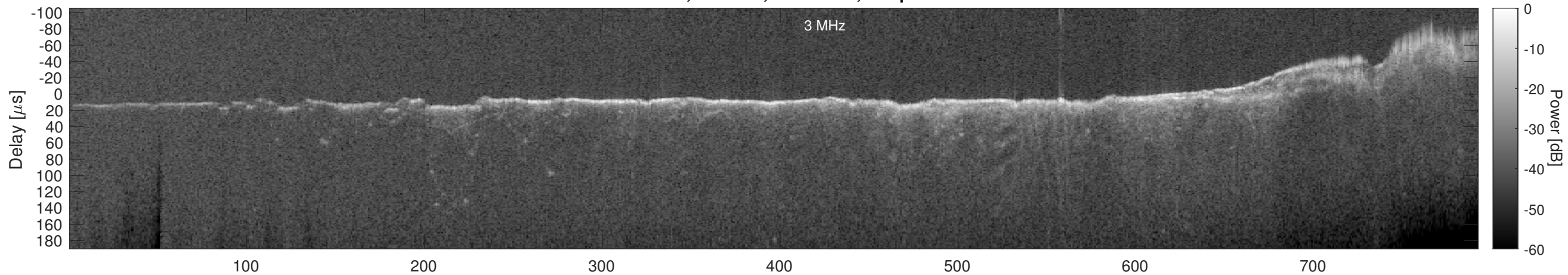
Orbit 2619, Window, Channel 2, Optimized
