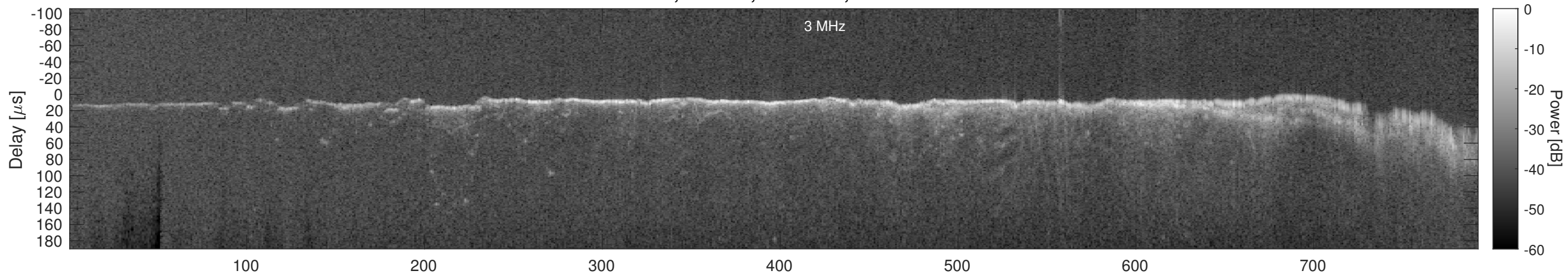
Orbit 2619, Window, Channel 2, Chapman
