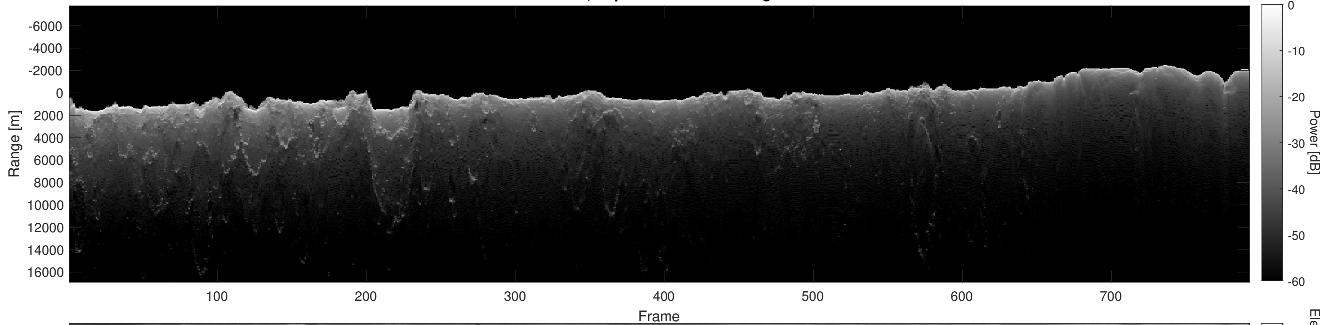
Orbit 2619, Depth-Corrected Cluttergram
