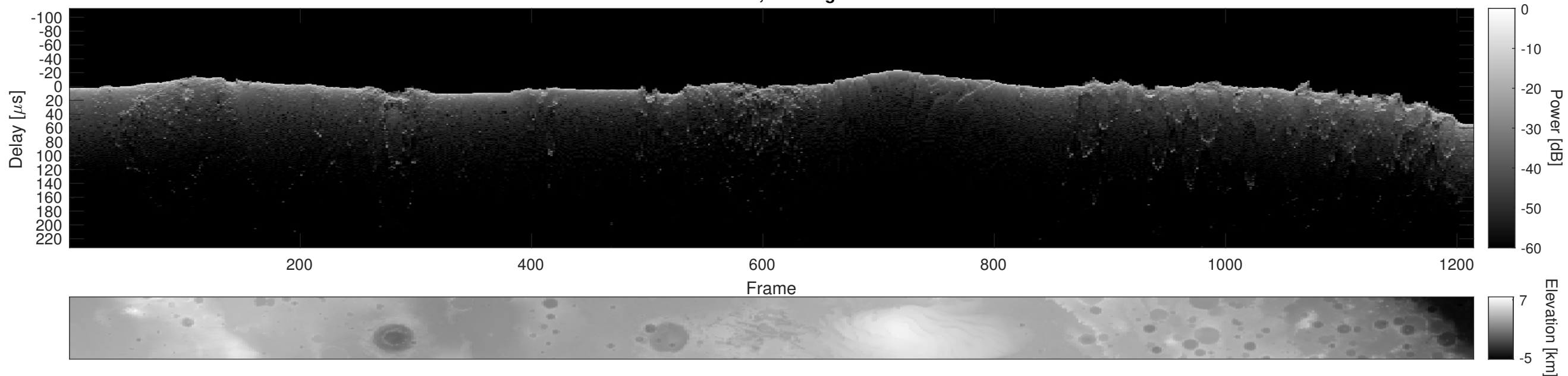
Orbit 2620, Cluttergram
