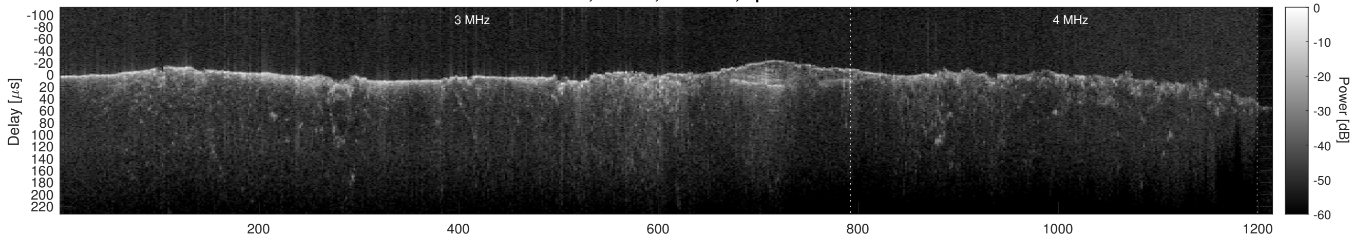
Orbit 2620, Cluttergram
