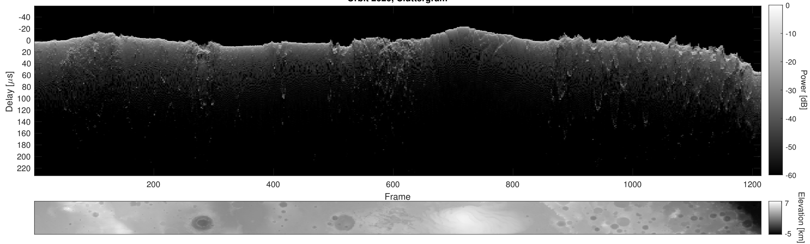
Orbit 2620, Cluttergram
