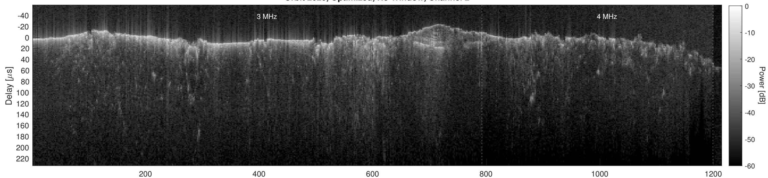
Orbit 2620, Cluttergram
