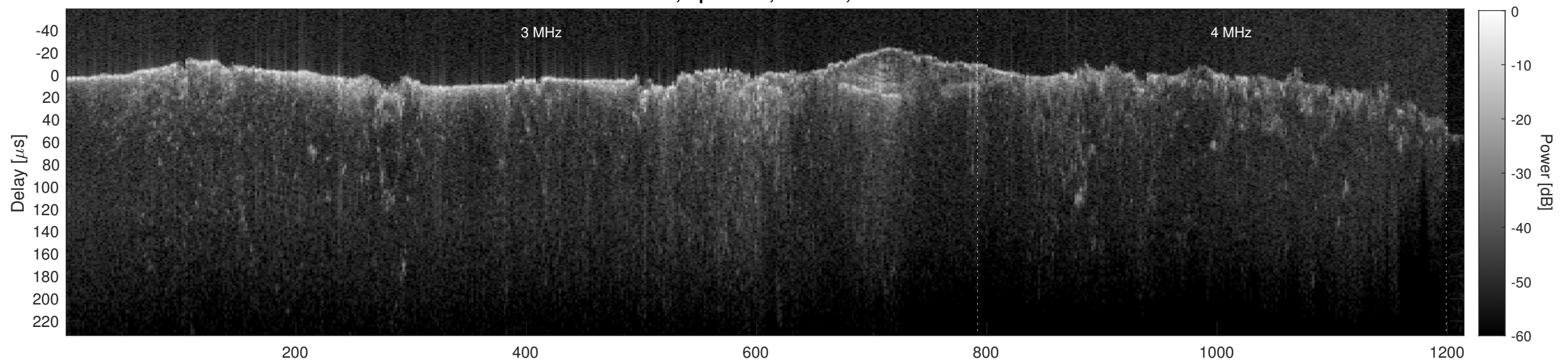
Orbit 2620, Cluttergram
