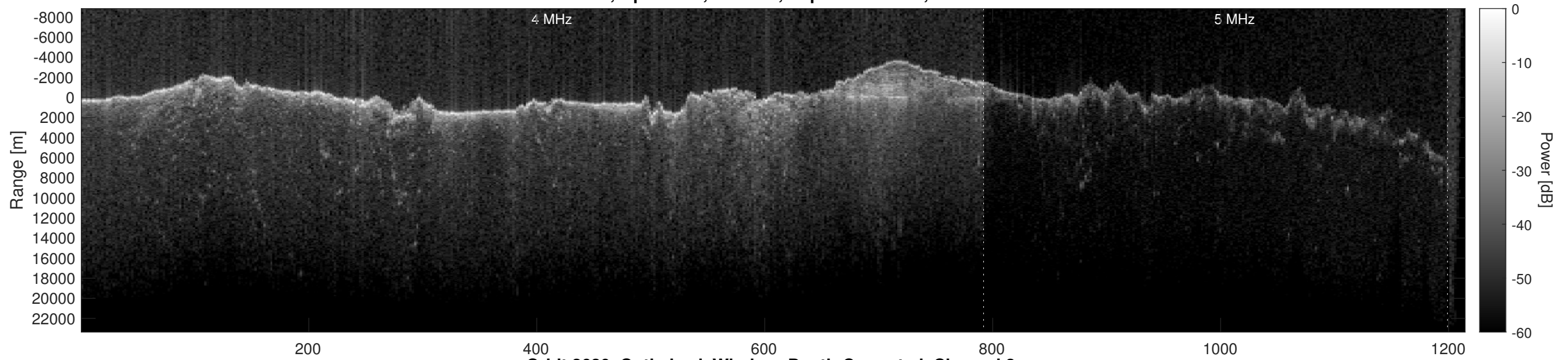
Orbit 2620, Optimized, Window, Depth-Corrected, Channel 2
