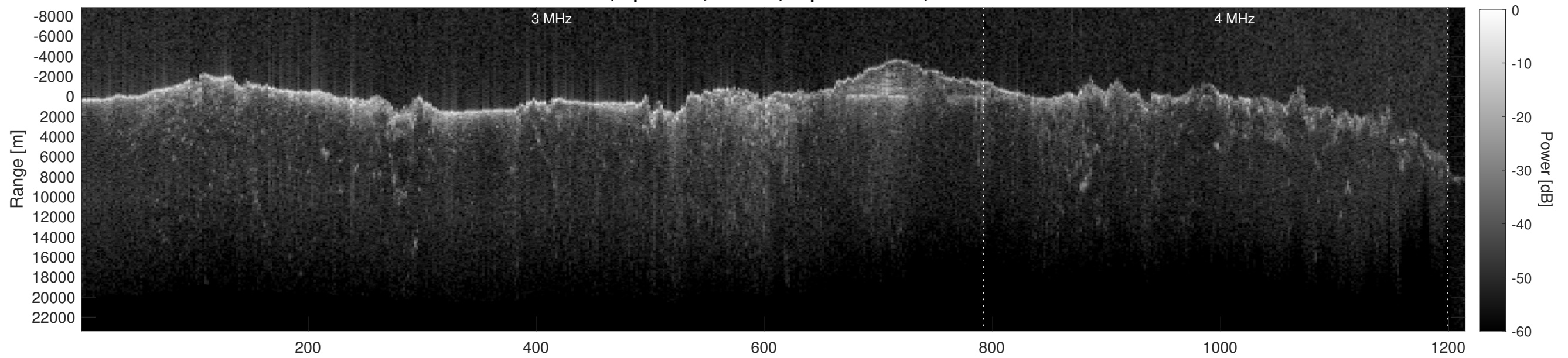
Orbit 2620, Depth-Corrected Cluttergram
