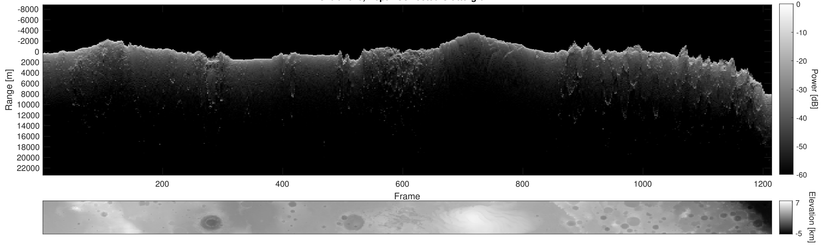
Orbit 2620, Depth-Corrected Cluttergram
