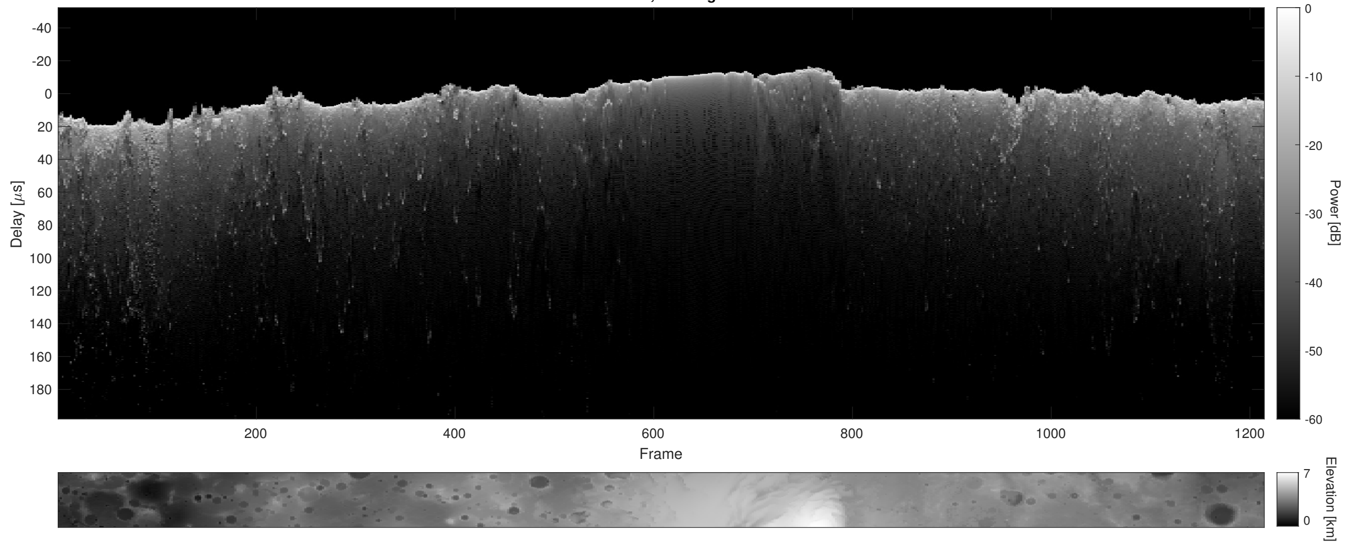
Orbit 2621, Cluttergram
