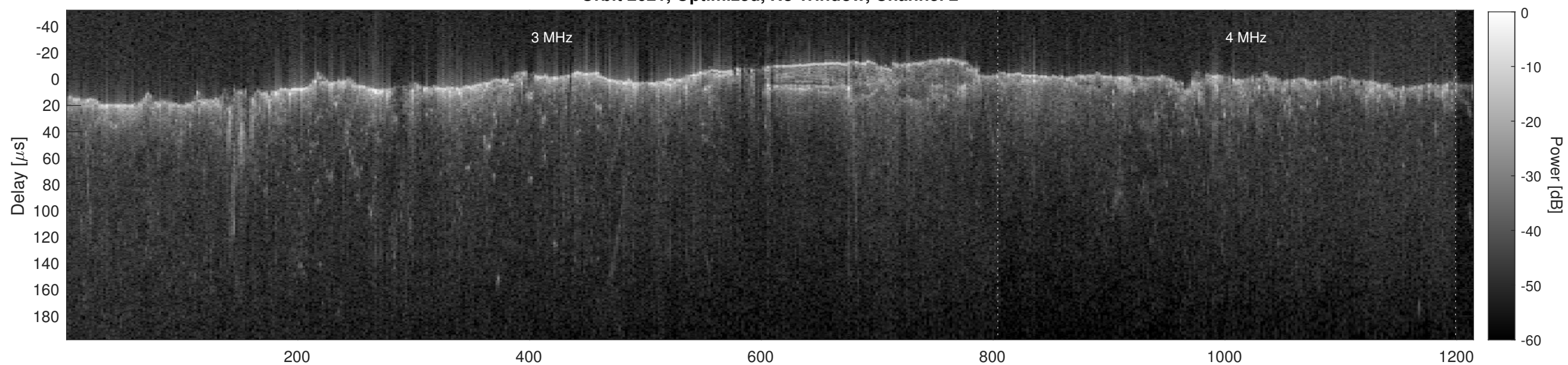
Orbit 2621, Cluttergram
