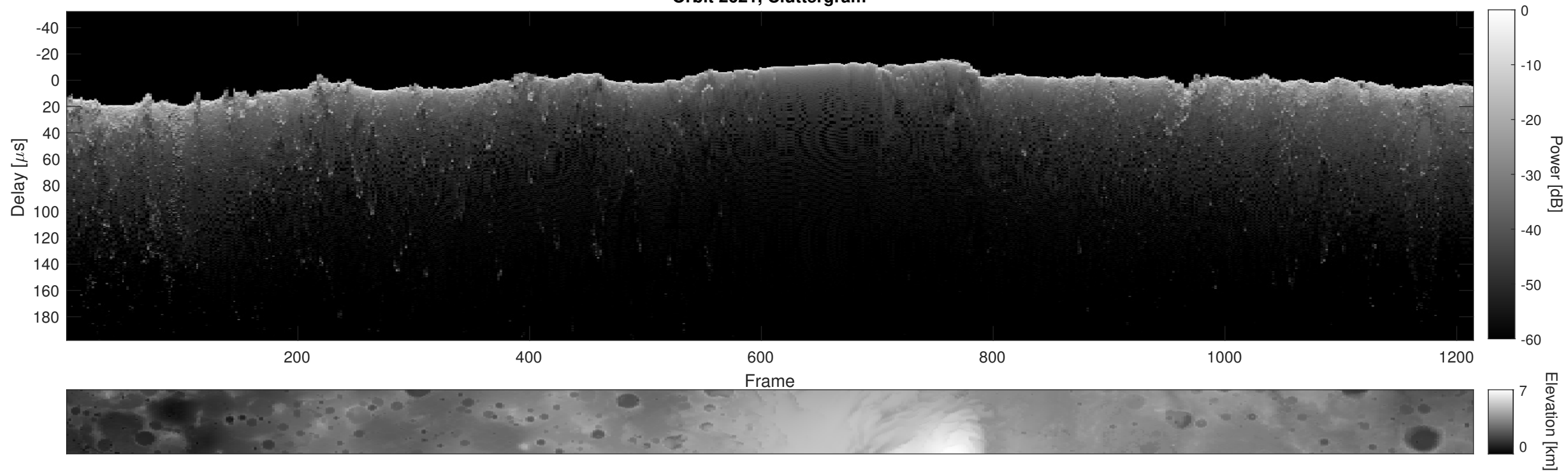
Orbit 2621, Cluttergram
