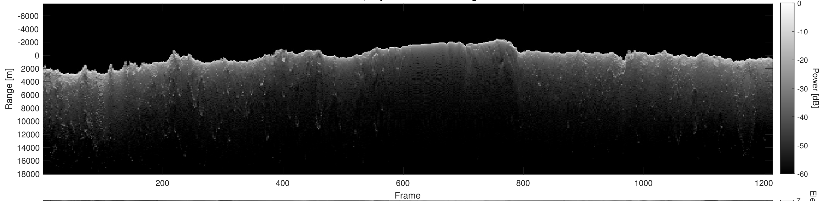
Orbit 2621, Depth-Corrected Cluttergram
