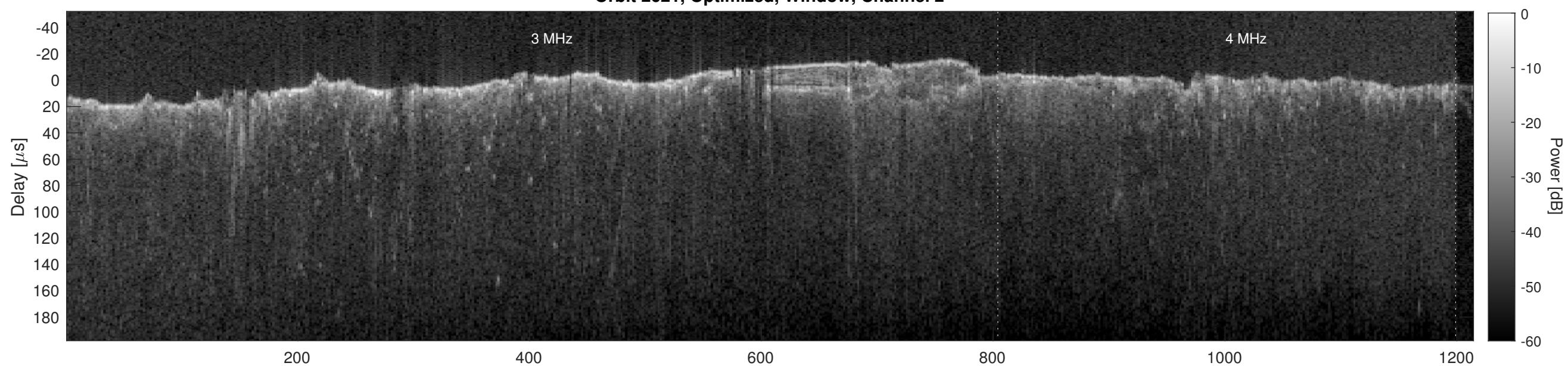
Orbit 2621, Cluttergram
