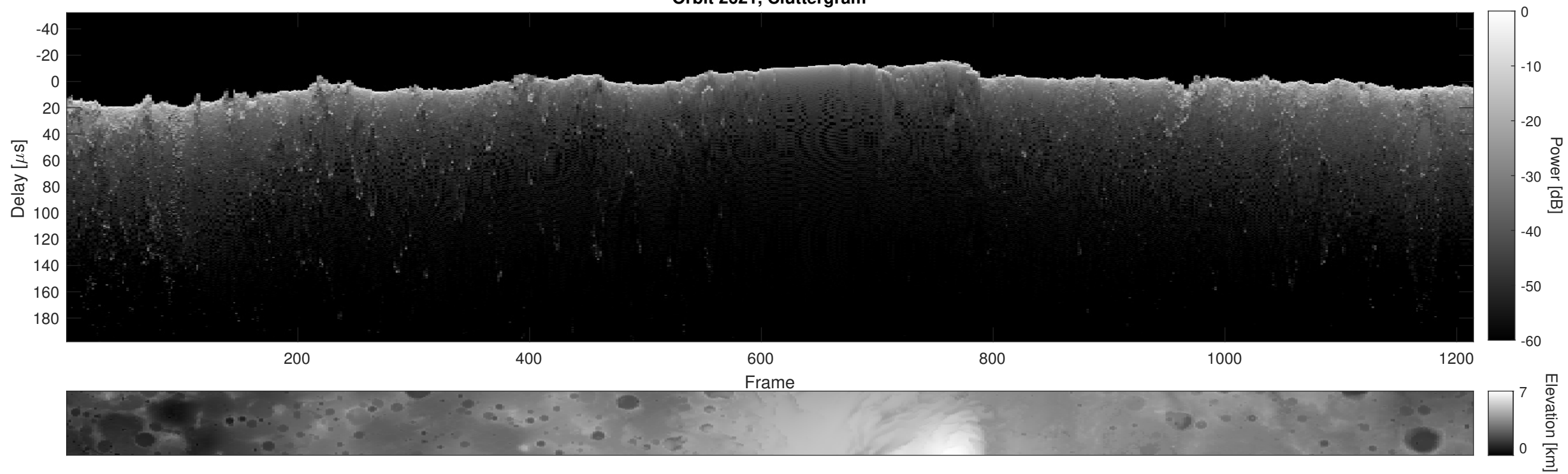
Orbit 2621, Cluttergram
