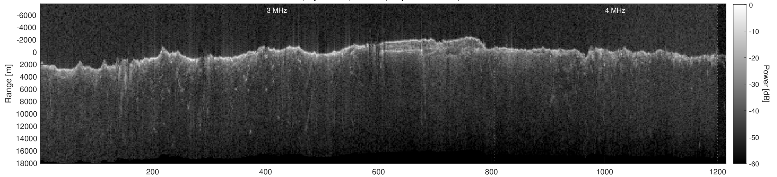
Orbit 2621, Depth-Corrected Cluttergram
