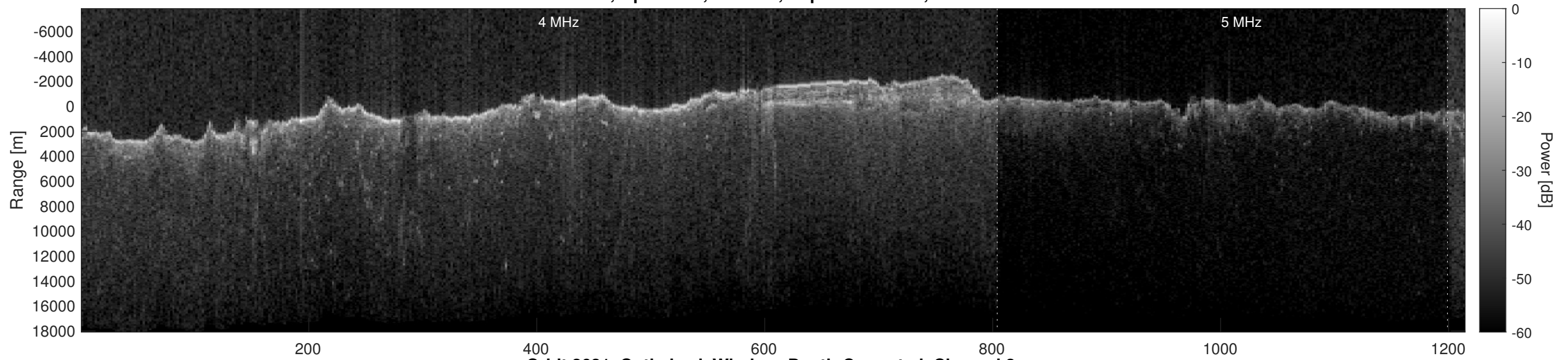
Orbit 2621, Optimized, Window, Depth-Corrected, Channel 2
