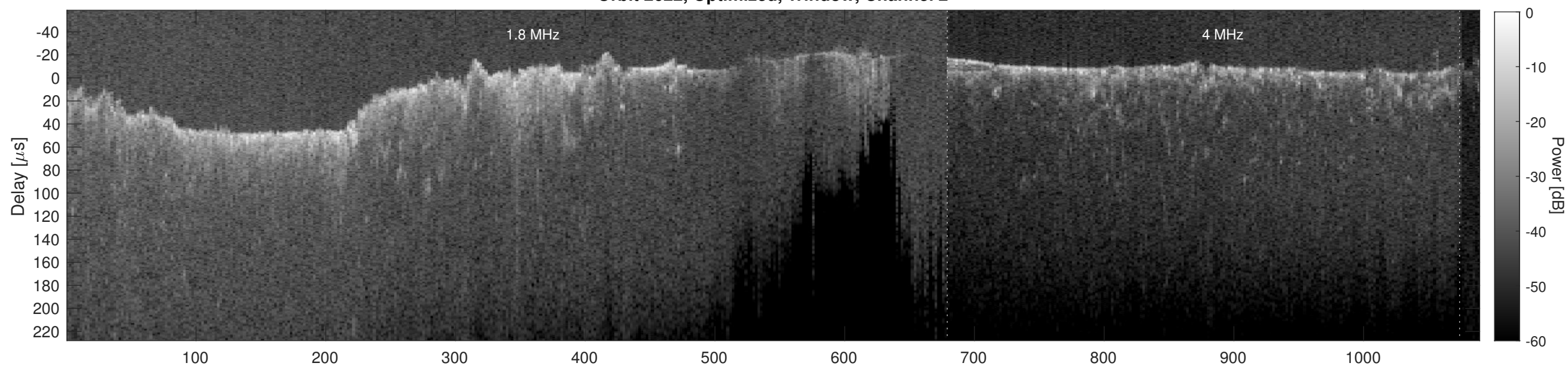
Orbit 2622, Cluttergram
