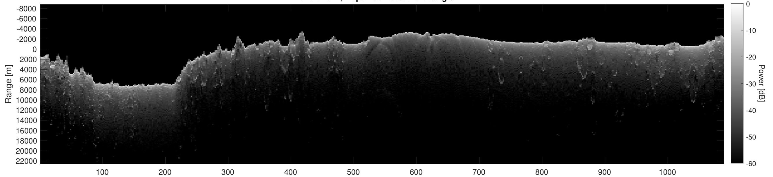
Orbit 2622, Depth-Corrected Cluttergram
