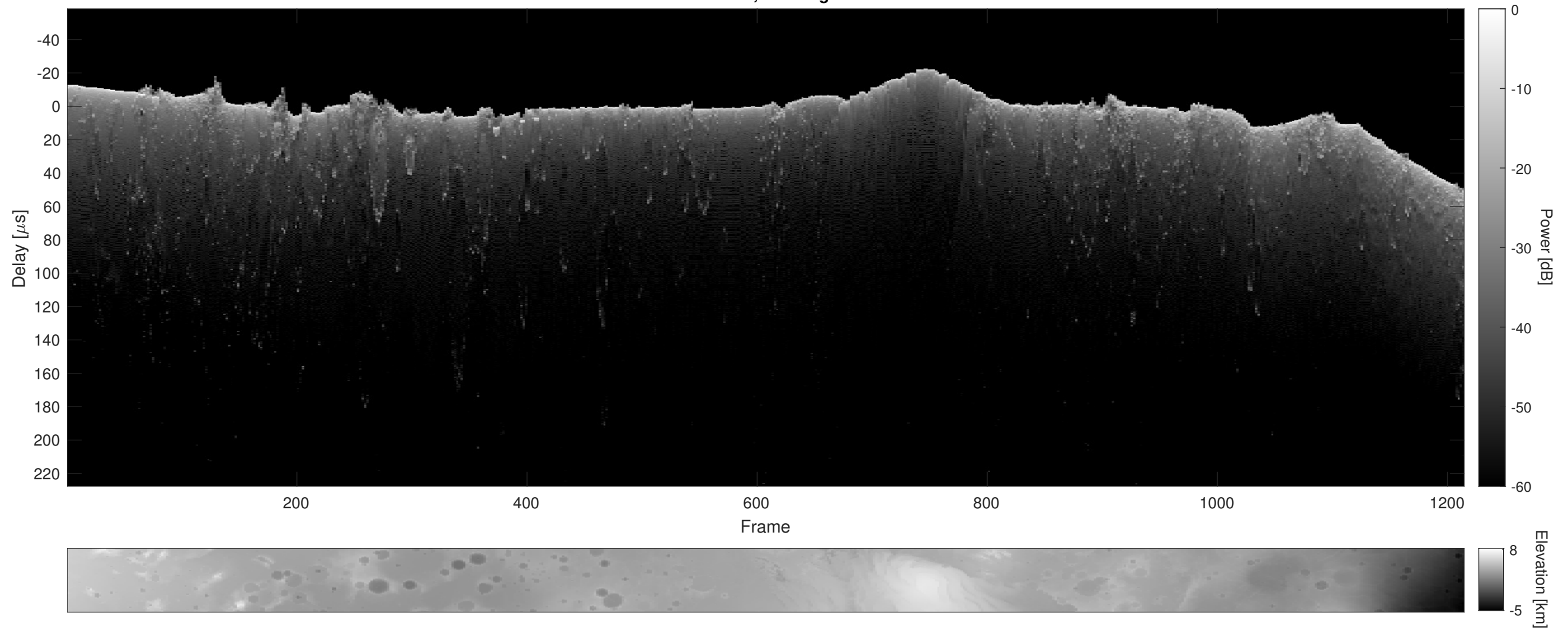
Orbit 2624, Cluttergram
