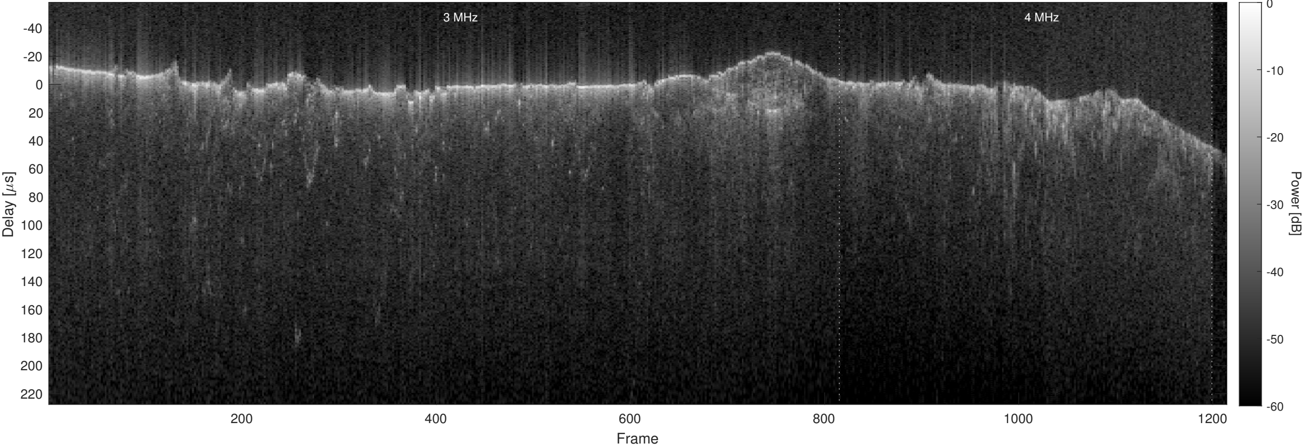
Orbit 2624, Optimized, No Window, Channel 2
