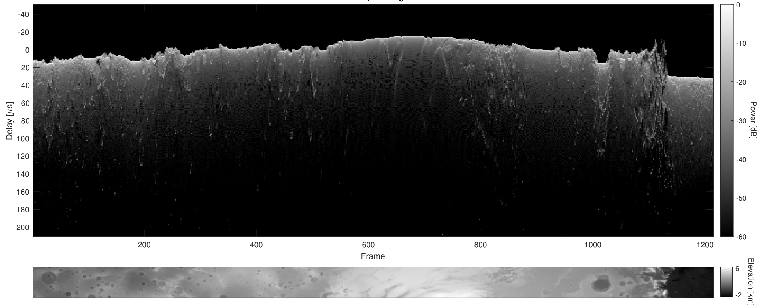
Orbit 2625, Cluttergram
