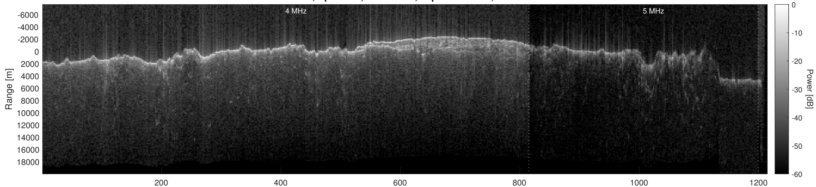
Orbit 2625, Optimized, No Window, Depth-Corrected, Channel 2
