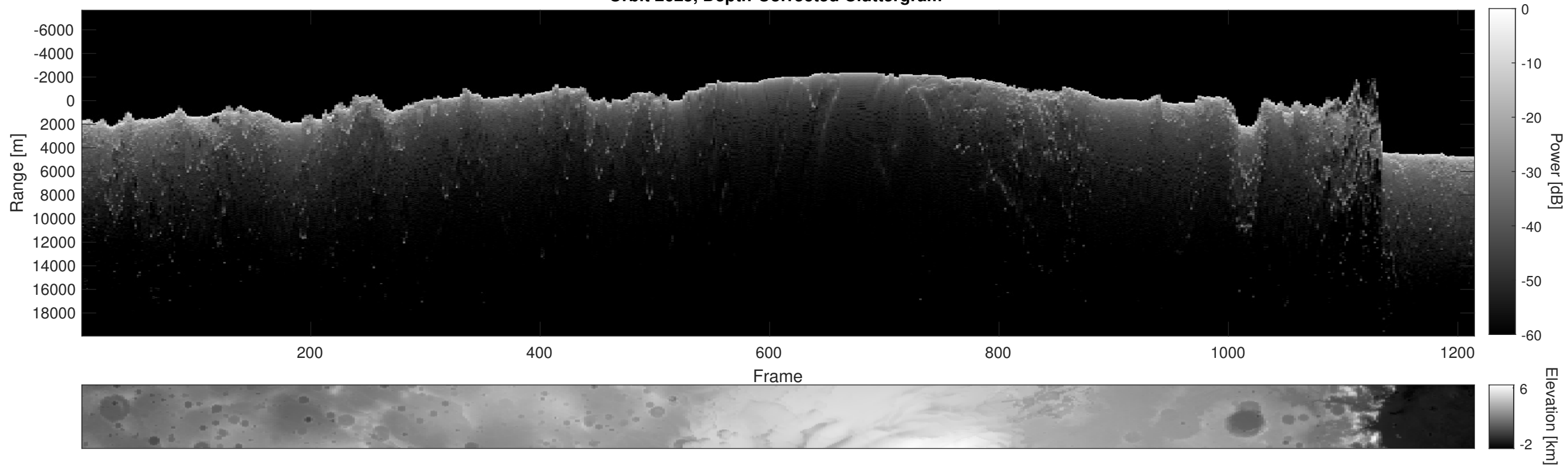
Orbit 2625, Depth-Corrected Cluttergram
