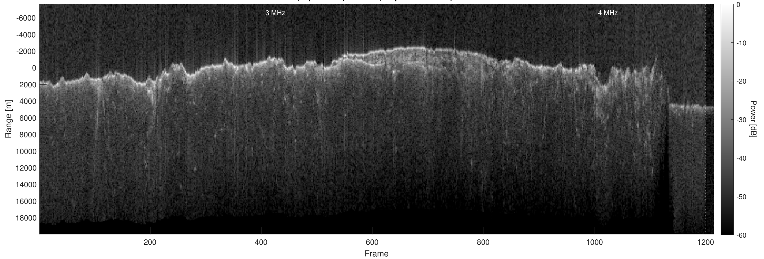
Orbit 2625, Optimized, Window, Depth-Corrected, Channel 2
