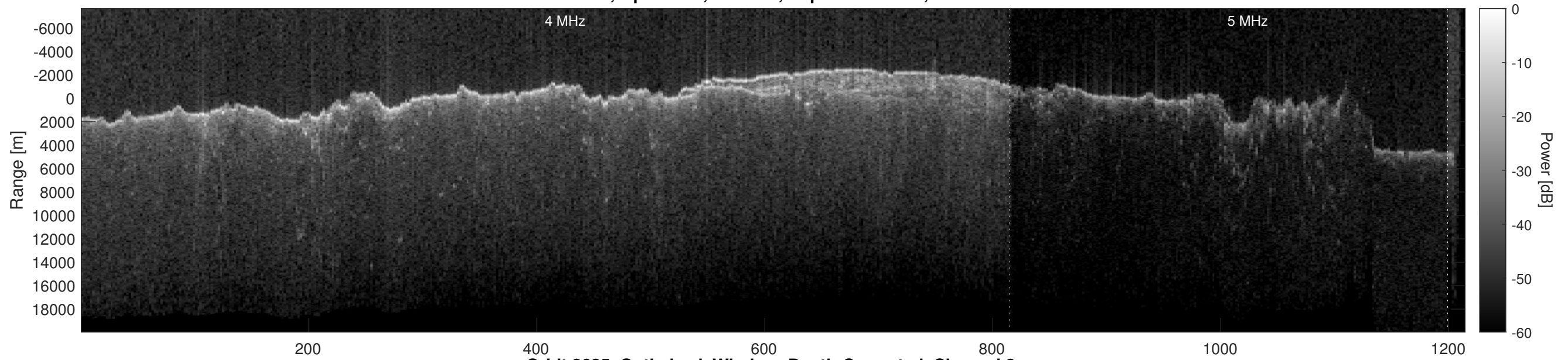
Orbit 2625, Optimized, Window, Depth-Corrected, Channel 2
