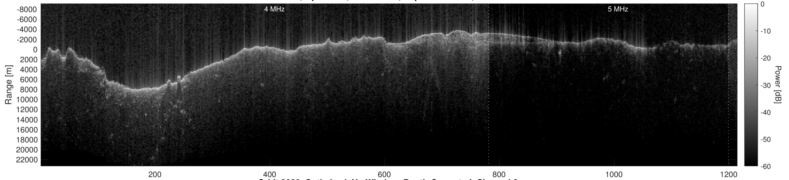
Orbit 2626, Optimized, No Window, Depth-Corrected, Channel 2
