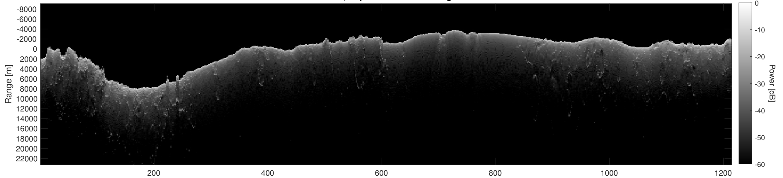
Orbit 2626, Depth-Corrected Cluttergram
