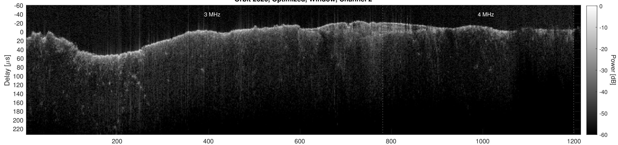
Orbit 2626, Cluttergram
